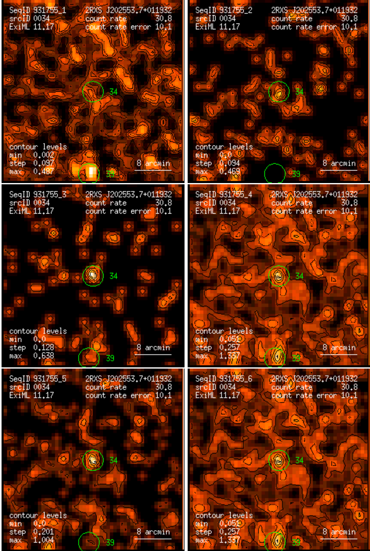
Figure 34: RASS 931755: detection 0034: band rate images, Gaussian filter: (1) PSPC channels 11 – 41, (2) 52 – 90, (3) 91 – 201, (4) 11 – 235, (5) 52 – 201, (6) 11 – 201. Broad band rates in counts/ks. Band rate contour levels in counts/ks/arcmin 2 .
