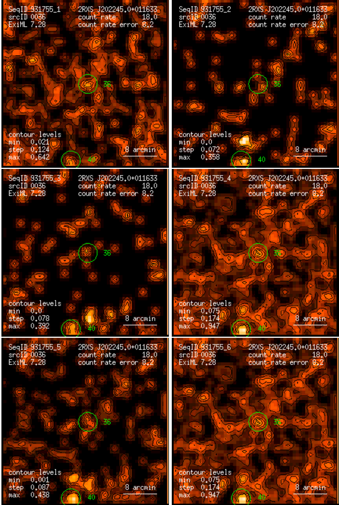
Figure 36: RASS 931755: detection 0036: band rate images, Gaussian filter: (1) PSPC channels 11 – 41, (2) 52 – 90, (3) 91 – 201, (4) 11 – 235, (5) 52 – 201, (6) 11 – 201. Broad band rates in counts/ks. Band rate contour levels in counts/ks/arcmin 2 .
