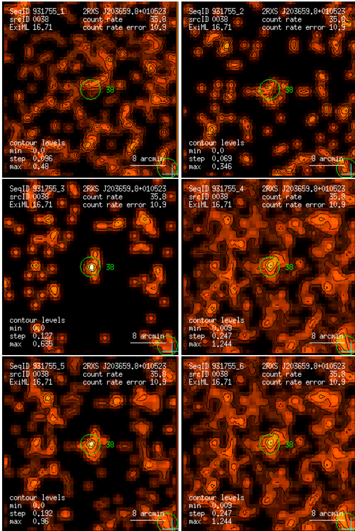
Figure 38: RASS 931755: detection 0038: band rate images, Gaussian filter: (1) PSPC channels 11 – 41, (2) 52 – 90, (3) 91 – 201, (4) 11 – 235, (5) 52 – 201, (6) 11 – 201. Broad band rates in counts/ks. Band rate contour levels in counts/ks/arcmin 2 .
