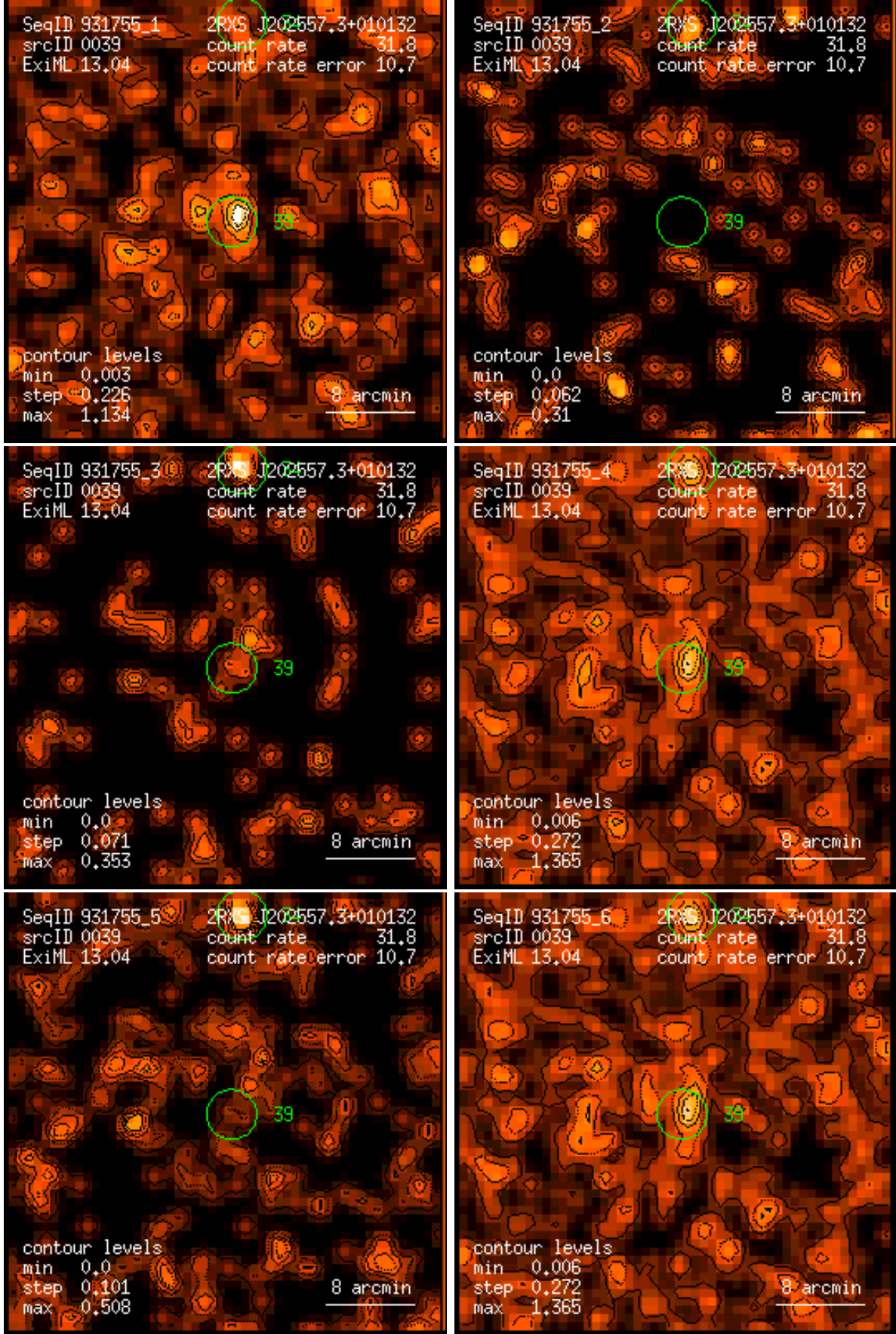
Figure 39: RASS 931755: detection 0039: band rate images, Gaussian filter: (1) PSPC channels 11 – 41, (2) 52 – 90, (3) 91 – 201, (4) 11 – 235, (5) 52 – 201, (6) 11 – 201. Broad band rates in counts/ks. Band rate contour levels in counts/ks/arcmin 2 .
