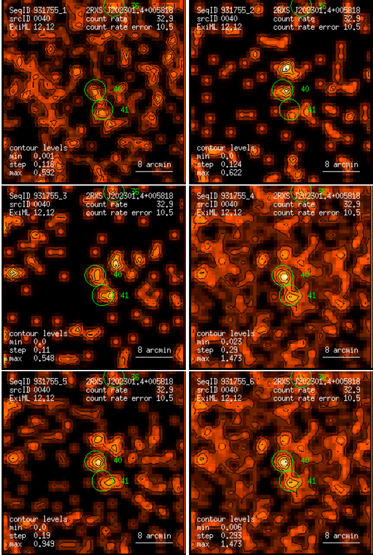
Figure 40: RASS 931755: detection 0040: band rate images, Gaussian filter: (1) PSPC channels 11 – 41, (2) 52 – 90, (3) 91 – 201, (4) 11 – 235, (5) 52 – 201, (6) 11 – 201. Broad band rates in counts/ks. Band rate contour levels in counts/ks/arcmin 2 .
