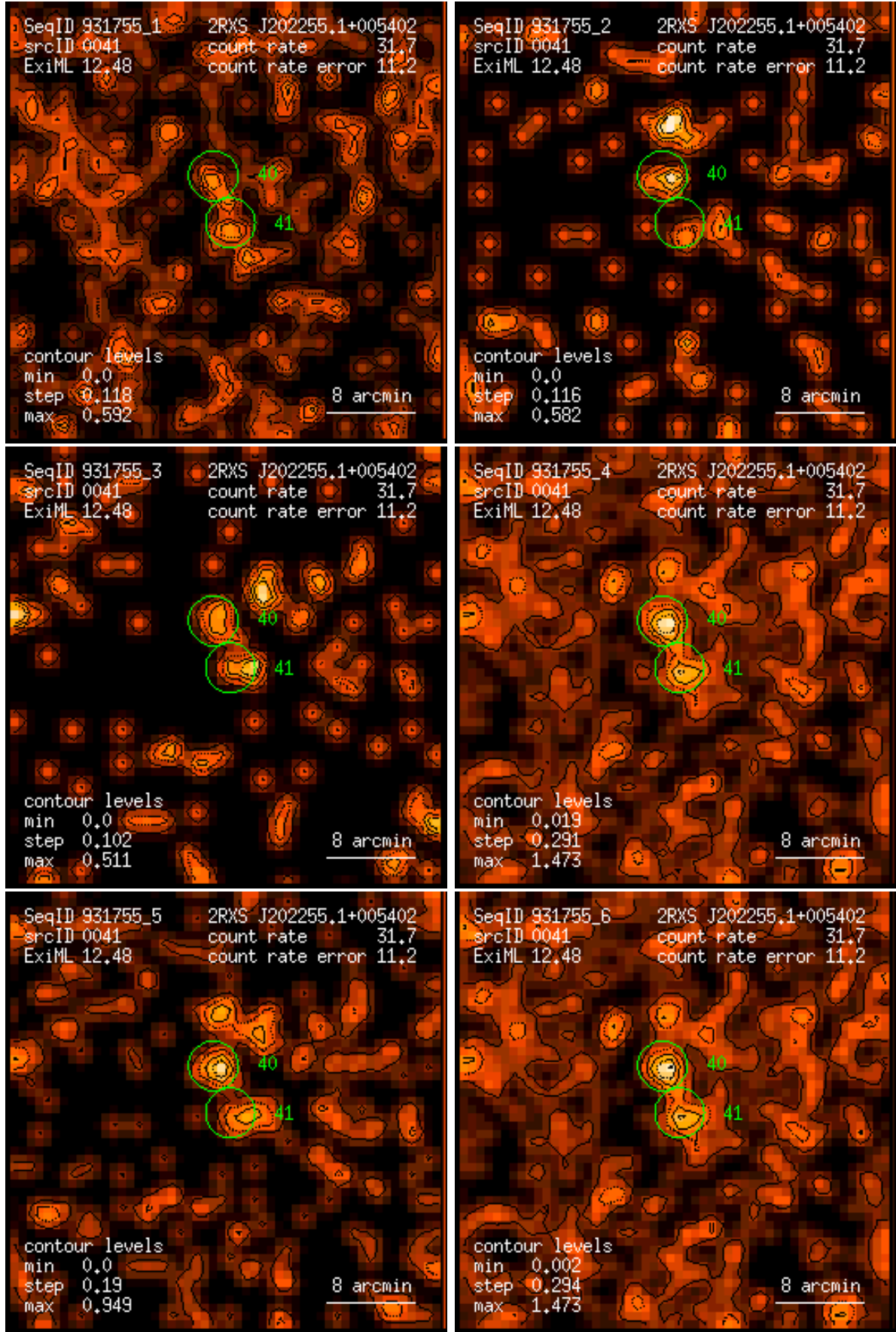
Figure 41: RASS 931755: detection 0041: band rate images, Gaussian filter: (1) PSPC channels 11 – 41, (2) 52 – 90, (3) 91 – 201, (4) 11 – 235, (5) 52 – 201, (6) 11 – 201. Broad band rates in counts/ks. Band rate contour levels in counts/ks/arcmin 2 .
