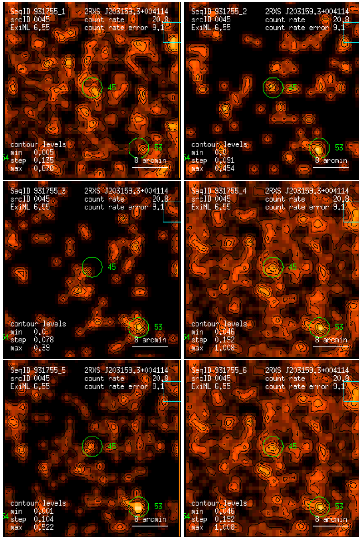
Figure 45: RASS 931755: detection 0045: band rate images, Gaussian filter: (1) PSPC channels 11 – 41, (2) 52 – 90, (3) 91 – 201, (4) 11 – 235, (5) 52 – 201, (6) 11 – 201. Broad band rates in counts/ks. Band rate contour levels in counts/ks/arcmin 2 .
