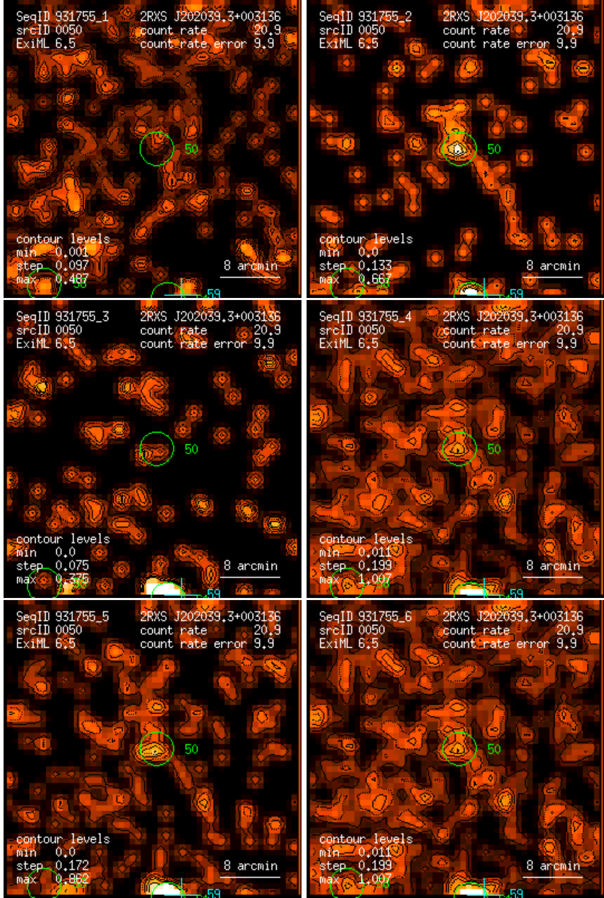
Figure 50: RASS 931755: detection 0050: band rate images, Gaussian filter: (1) PSPC channels 11 – 41, (2) 52 – 90, (3) 91 – 201, (4) 11 – 235, (5) 52 – 201, (6) 11 – 201. Broad band rates in counts/ks. Band rate contour levels in counts/ks/arcmin 2 .
