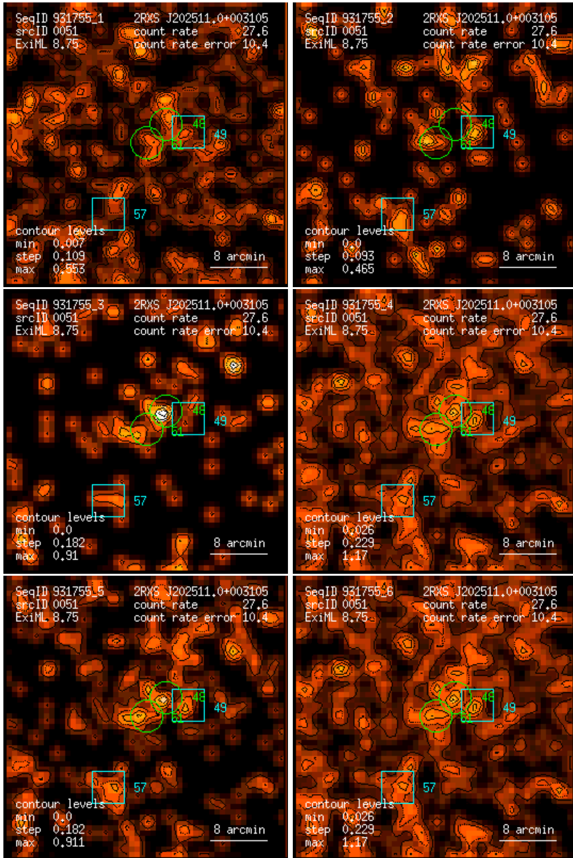
Figure 51: RASS 931755: detection 0051: band rate images, Gaussian filter: (1) PSPC channels 11 – 41, (2) 52 – 90, (3) 91 – 201, (4) 11 – 235, (5) 52 – 201, (6) 11 – 201. Broad band rates in counts/ks. Band rate contour levels in counts/ks/arcmin 2 .
