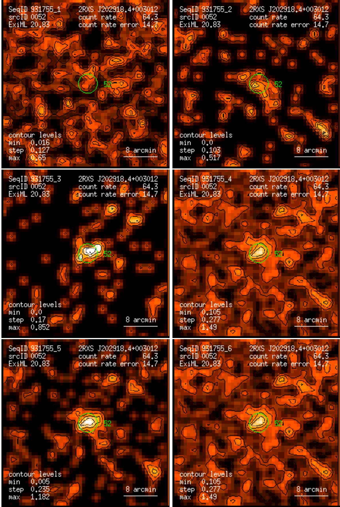
Figure 52: RASS 931755: detection 0052: band rate images, Gaussian filter: (1) PSPC channels 11 – 41, (2) 52 – 90, (3) 91 – 201, (4) 11 – 235, (5) 52 – 201, (6) 11 – 201. Broad band rates in counts/ks. Band rate contour levels in counts/ks/arcmin 2 .
