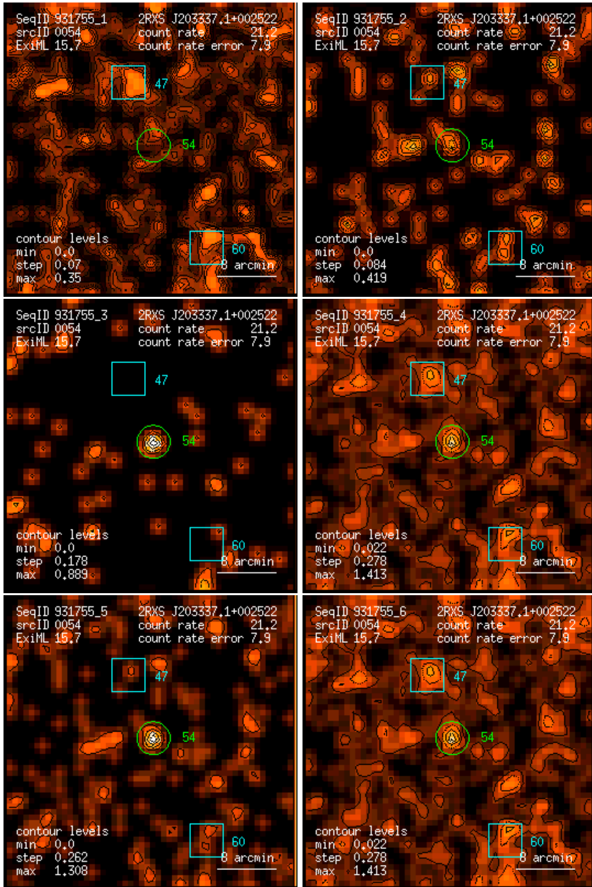
Figure 54: RASS 931755: detection 0054: band rate images, Gaussian filter: (1) PSPC channels 11 – 41, (2) 52 – 90, (3) 91 – 201, (4) 11 – 235, (5) 52 – 201, (6) 11 – 201. Broad band rates in counts/ks. Band rate contour levels in counts/ks/arcmin 2 .
