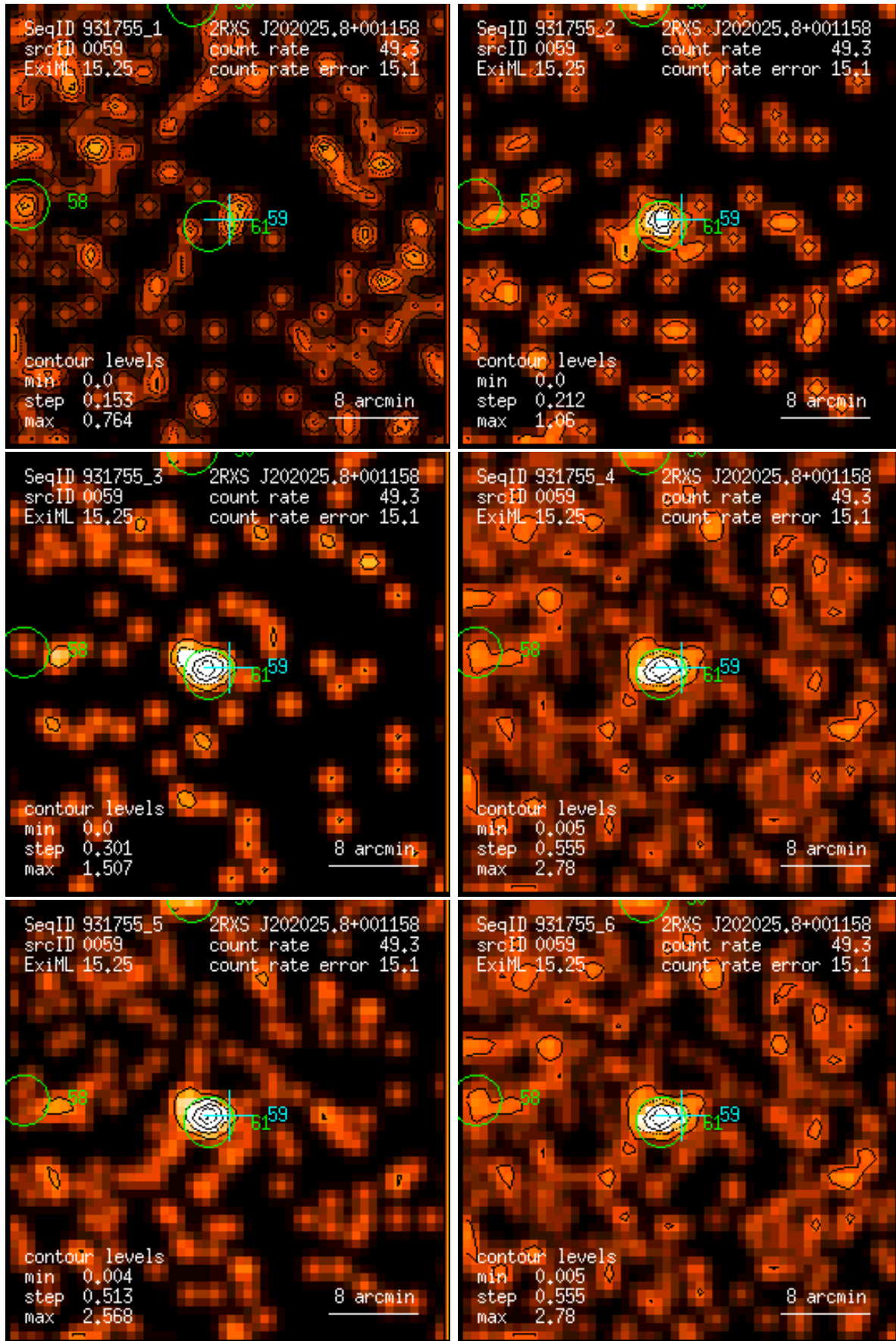
Figure 59: RASS 931755: detection 0059: band rate images, Gaussian filter: (1) PSPC channels 11 – 41, (2) 52 – 90, (3) 91 – 201, (4) 11 – 235, (5) 52 – 201, (6) 11 – 201. Broad band rates in counts/ks. Band rate contour levels in counts/ks/arcmin 2 .
