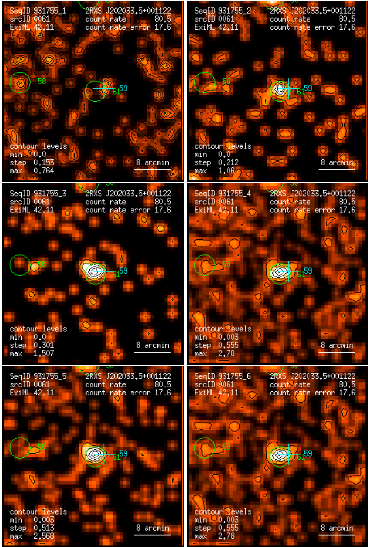
Figure 61: RASS 931755: detection 0061: band rate images, Gaussian filter: (1) PSPC channels 11 – 41, (2) 52 – 90, (3) 91 – 201, (4) 11 – 235, (5) 52 – 201, (6) 11 – 201. Broad band rates in counts/ks. Band rate contour levels in counts/ks/arcmin 2 .
