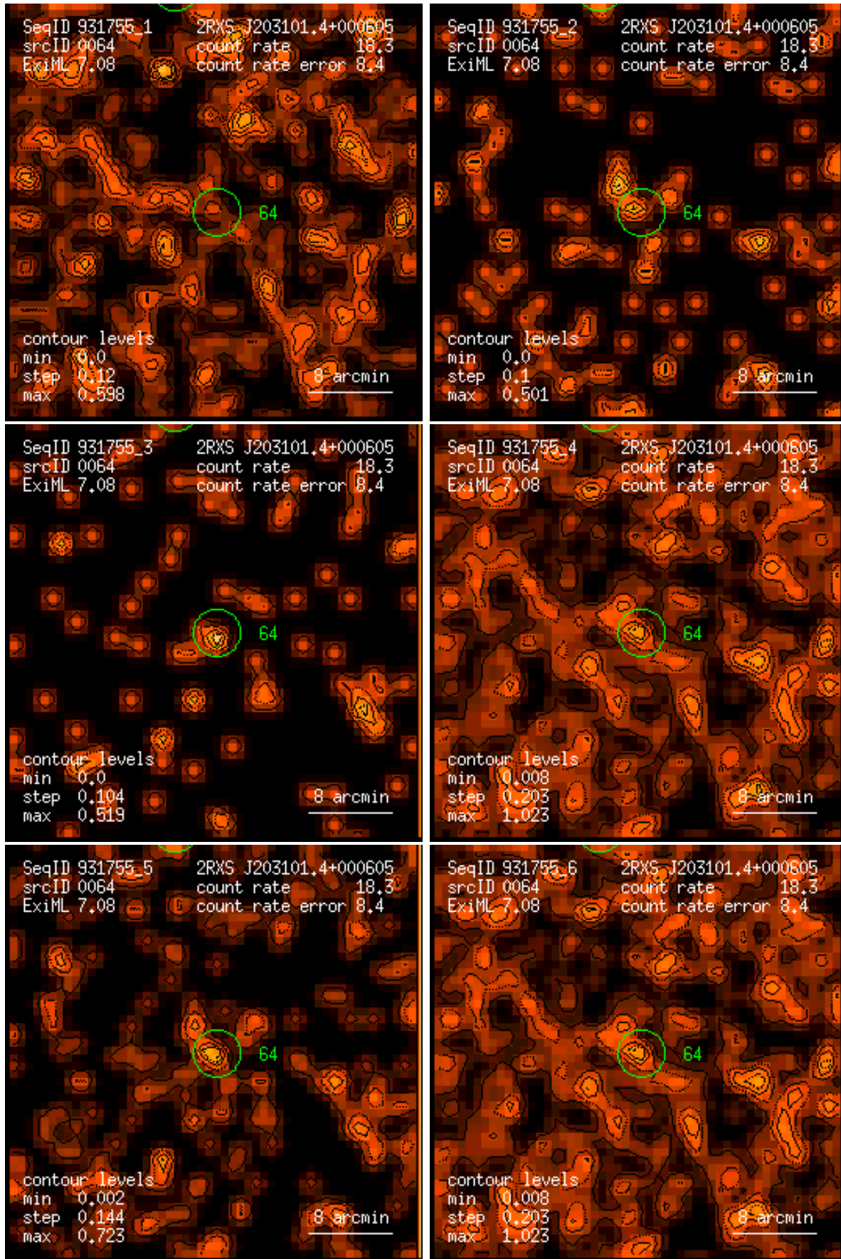
Figure 64: RASS 931755: detection 0064: band rate images, Gaussian filter: (1) PSPC channels 11 – 41, (2) 52 – 90, (3) 91 – 201, (4) 11 – 235, (5) 52 – 201, (6) 11 – 201. Broad band rates in counts/ks. Band rate contour levels in counts/ks/arcmin 2 .
