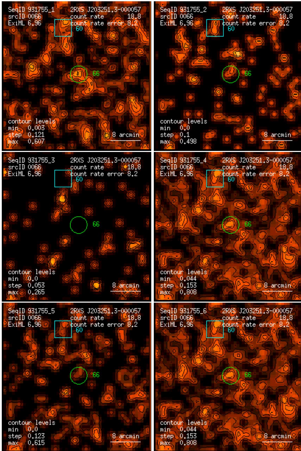
Figure 66: RASS 931755: detection 0066: band rate images, Gaussian filter: (1) PSPC channels 11 – 41, (2) 52 – 90, (3) 91 – 201, (4) 11 – 235, (5) 52 – 201, (6) 11 – 201. Broad band rates in counts/ks. Band rate contour levels in counts/ks/arcmin 2 .
