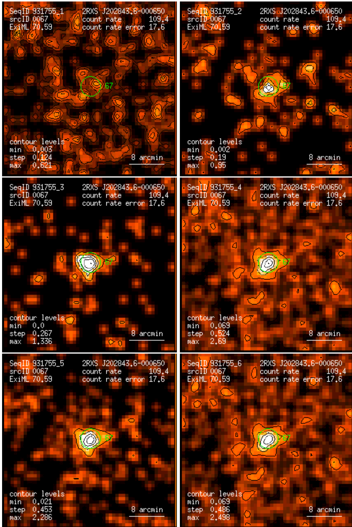
Figure 67: RASS 931755: detection 0067: band rate images, Gaussian filter: (1) PSPC channels 11 – 41, (2) 52 – 90, (3) 91 – 201, (4) 11 – 235, (5) 52 – 201, (6) 11 – 201. Broad band rates in counts/ks. Band rate contour levels in counts/ks/arcmin 2 .
