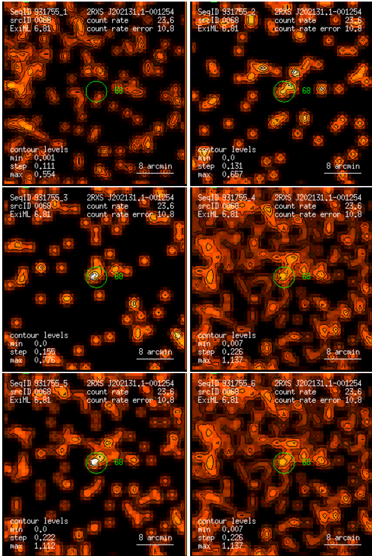
Figure 68: RASS 931755: detection 0068: band rate images, Gaussian filter: (1) PSPC channels 11 – 41, (2) 52 – 90, (3) 91 – 201, (4) 11 – 235, (5) 52 – 201, (6) 11 – 201. Broad band rates in counts/ks. Band rate contour levels in counts/ks/arcmin 2 .
