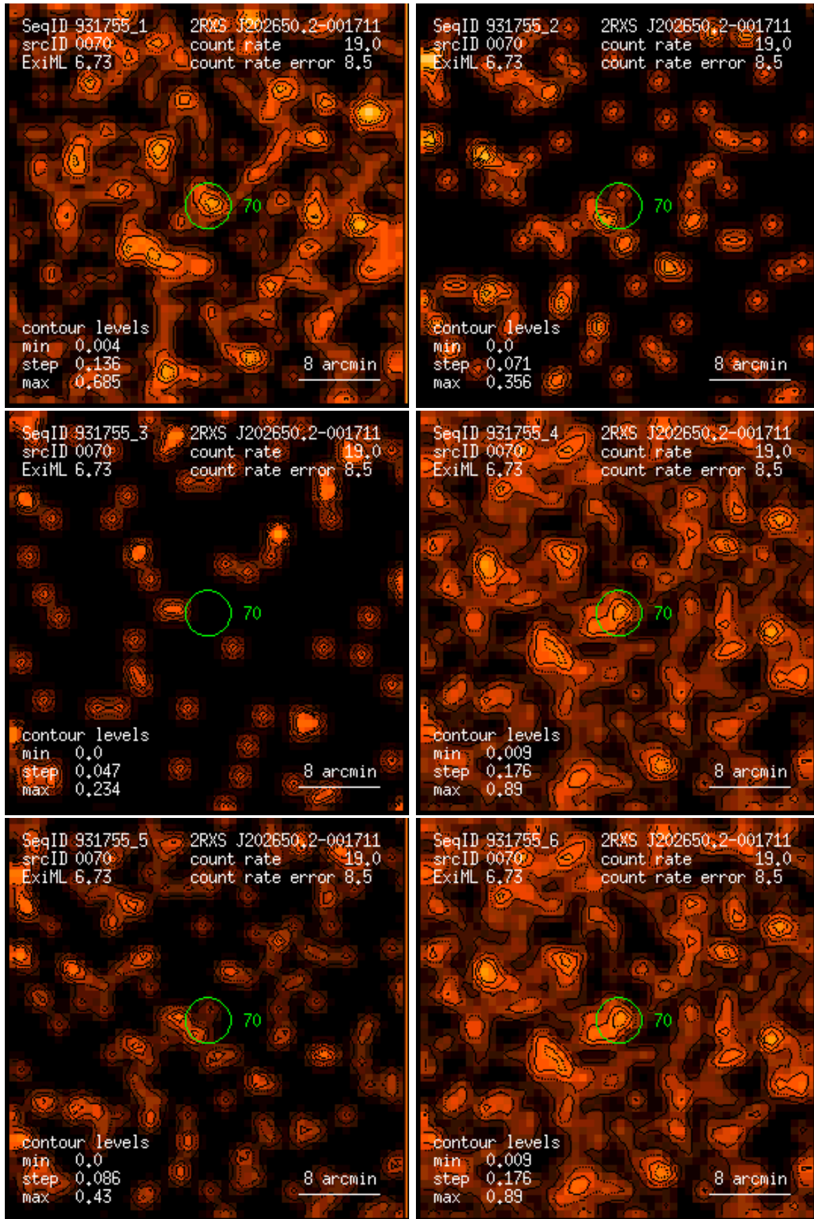
Figure 70: RASS 931755: detection 0070: band rate images, Gaussian filter: (1) PSPC channels 11 – 41, (2) 52 – 90, (3) 91 – 201, (4) 11 – 235, (5) 52 – 201, (6) 11 – 201. Broad band rates in counts/ks. Band rate contour levels in counts/ks/arcmin 2 .
