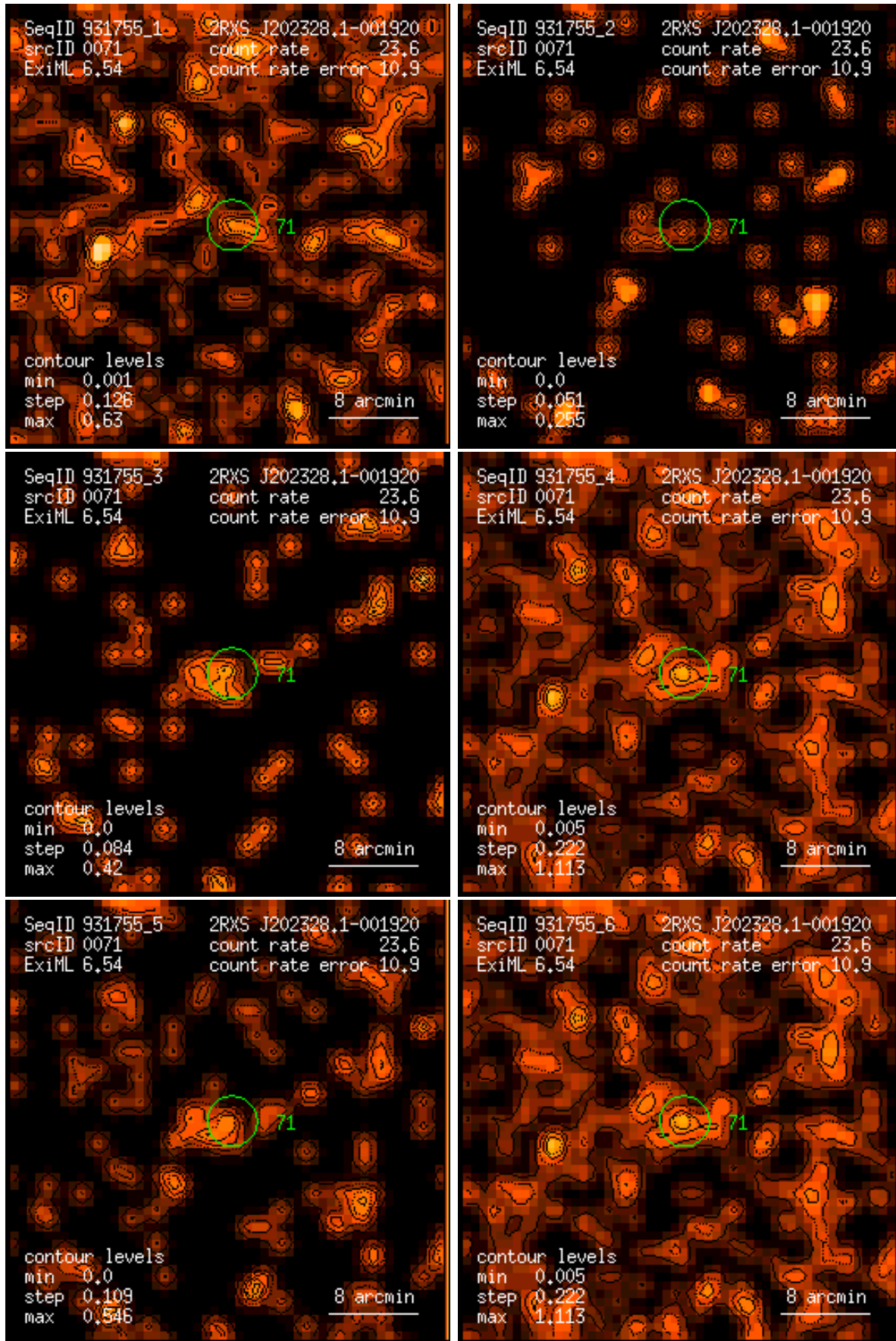
Figure 71: RASS 931755: detection 0071: band rate images, Gaussian filter: (1) PSPC channels 11 – 41, (2) 52 – 90, (3) 91 – 201, (4) 11 – 235, (5) 52 – 201, (6) 11 – 201. Broad band rates in counts/ks. Band rate contour levels in counts/ks/arcmin 2 .
