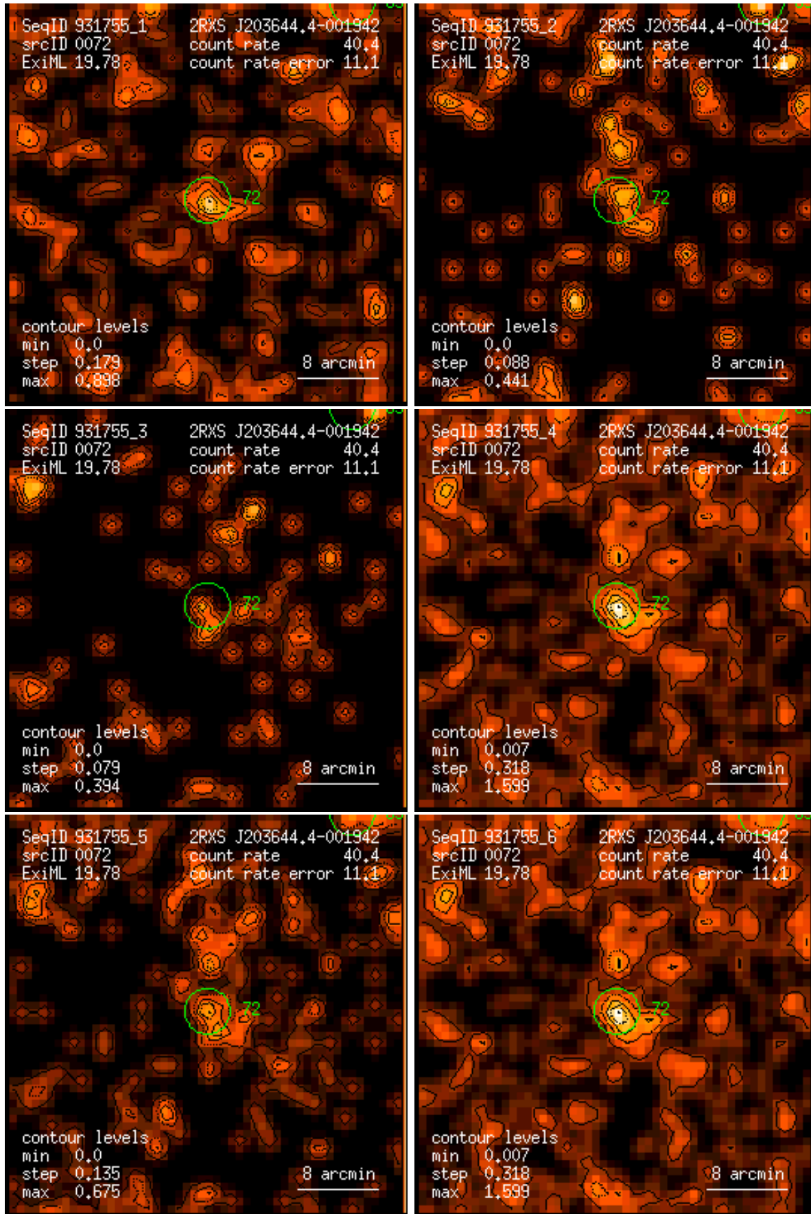
Figure 72: RASS 931755: detection 0072: band rate images, Gaussian filter: (1) PSPC channels 11 – 41, (2) 52 – 90, (3) 91 – 201, (4) 11 – 235, (5) 52 – 201, (6) 11 – 201. Broad band rates in counts/ks. Band rate contour levels in counts/ks/arcmin 2 .
