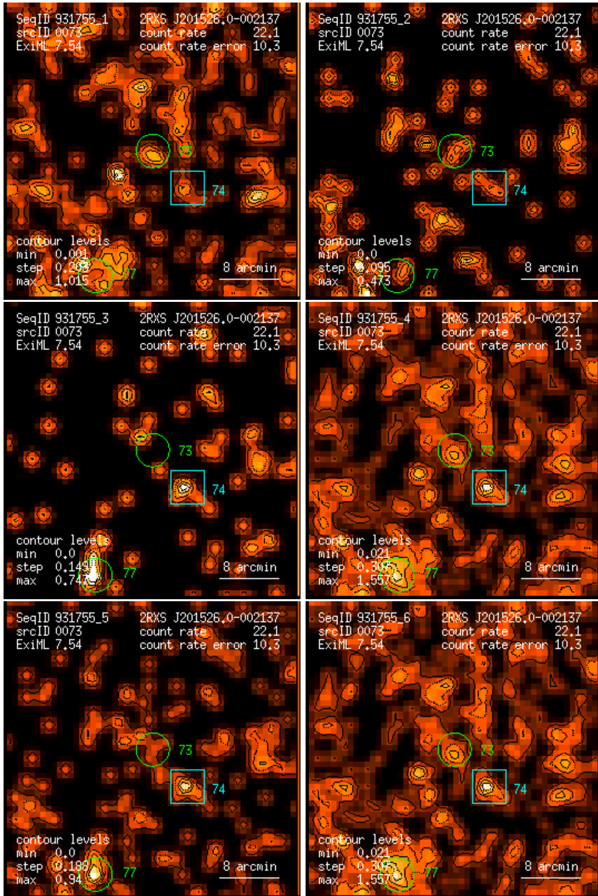
Figure 73: RASS 931755: detection 0073: band rate images, Gaussian filter: (1) PSPC channels 11 – 41, (2) 52 – 90, (3) 91 – 201, (4) 11 – 235, (5) 52 – 201, (6) 11 – 201. Broad band rates in counts/ks. Band rate contour levels in counts/ks/arcmin 2 .
