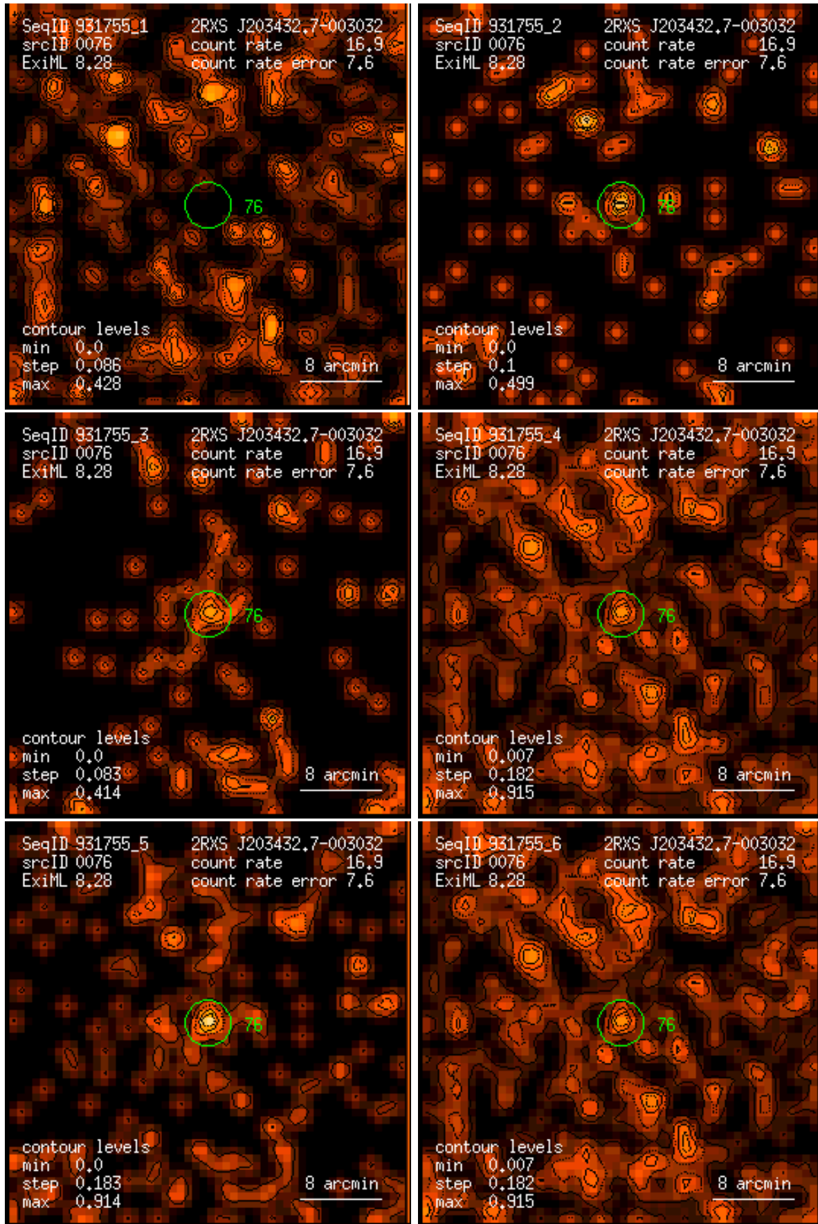
Figure 76: RASS 931755: detection 0076: band rate images, Gaussian filter: (1) PSPC channels 11 – 41, (2) 52 – 90, (3) 91 – 201, (4) 11 – 235, (5) 52 – 201, (6) 11 – 201. Broad band rates in counts/ks. Band rate contour levels in counts/ks/arcmin 2 .
