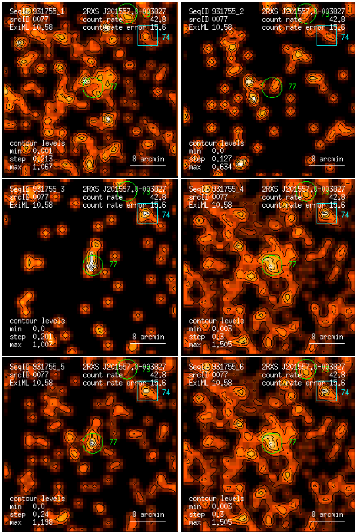
Figure 77: RASS 931755: detection 0077: band rate images, Gaussian filter: (1) PSPC channels 11 – 41, (2) 52 – 90, (3) 91 – 201, (4) 11 – 235, (5) 52 – 201, (6) 11 – 201. Broad band rates in counts/ks. Band rate contour levels in counts/ks/arcmin 2 .
