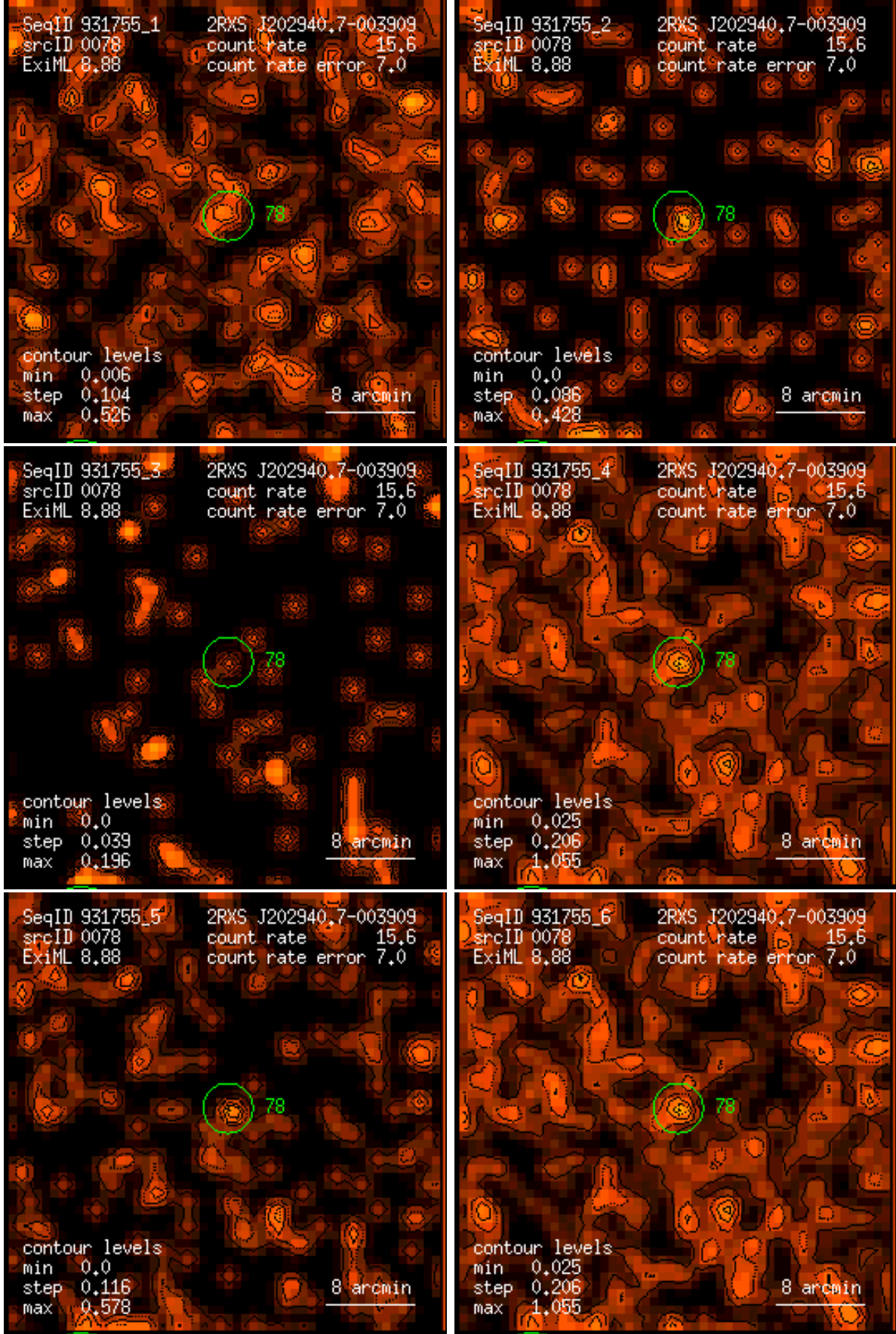
Figure 78: RASS 931755: detection 0078: band rate images, Gaussian filter: (1) PSPC channels 11 – 41, (2) 52 – 90, (3) 91 – 201, (4) 11 – 235, (5) 52 – 201, (6) 11 – 201. Broad band rates in counts/ks. Band rate contour levels in counts/ks/arcmin 2 .
