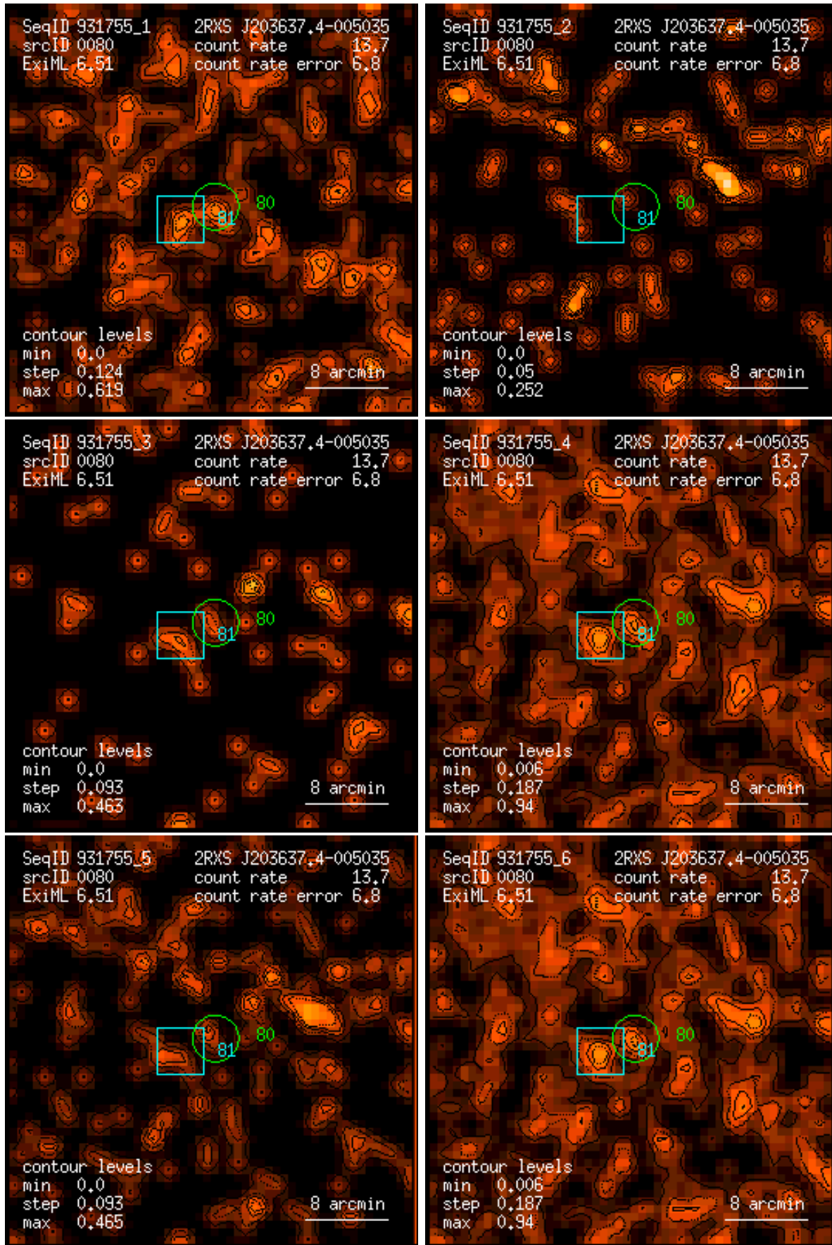
Figure 80: RASS 931755: detection 0080: band rate images, Gaussian filter: (1) PSPC channels 11 – 41, (2) 52 – 90, (3) 91 – 201, (4) 11 – 235, (5) 52 – 201, (6) 11 – 201. Broad band rates in counts/ks. Band rate contour levels in counts/ks/arcmin 2 .
