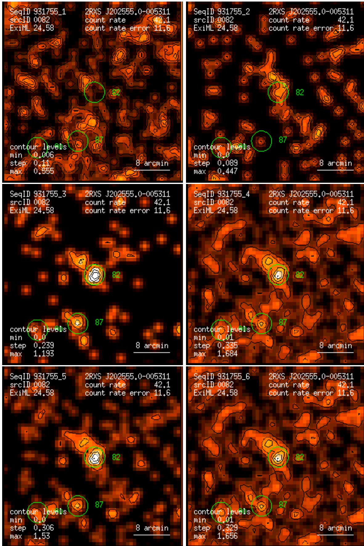
Figure 82: RASS 931755: detection 0082: band rate images, Gaussian filter: (1) PSPC channels 11 – 41, (2) 52 – 90, (3) 91 – 201, (4) 11 – 235, (5) 52 – 201, (6) 11 – 201. Broad band rates in counts/ks. Band rate contour levels in counts/ks/arcmin 2 .
