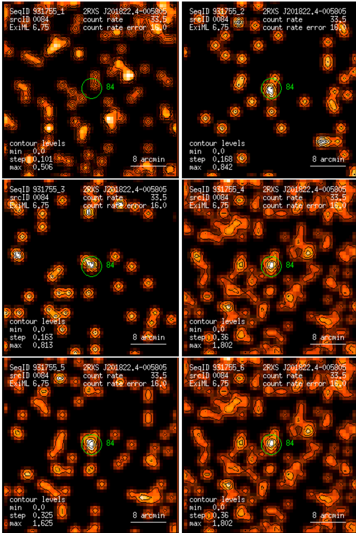
Figure 84: RASS 931755: detection 0084: band rate images, Gaussian filter: (1) PSPC channels 11 – 41, (2) 52 – 90, (3) 91 – 201, (4) 11 – 235, (5) 52 – 201, (6) 11 – 201. Broad band rates in counts/ks. Band rate contour levels in counts/ks/arcmin 2 .
