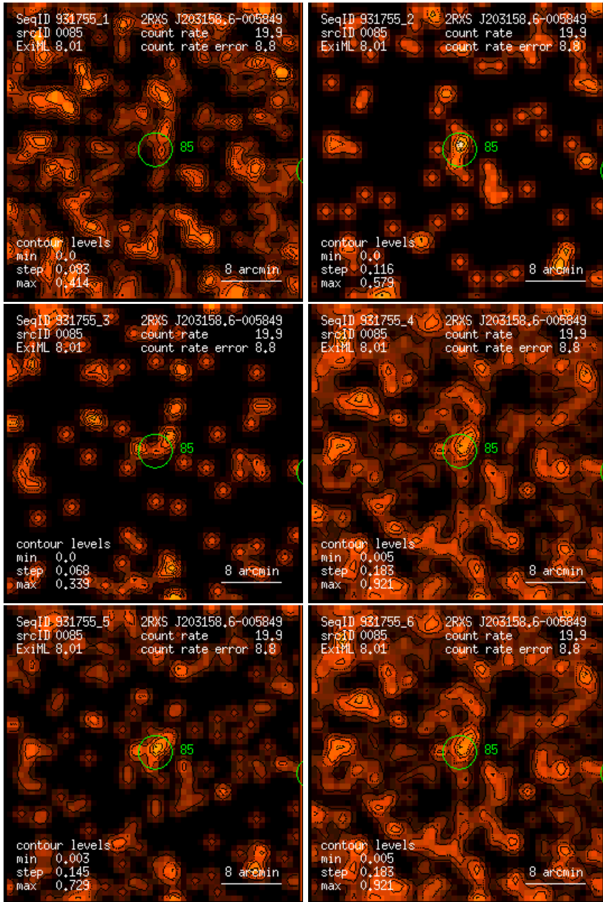
Figure 85: RASS 931755: detection 0085: band rate images, Gaussian filter: (1) PSPC channels 11 – 41, (2) 52 – 90, (3) 91 – 201, (4) 11 – 235, (5) 52 – 201, (6) 11 – 201. Broad band rates in counts/ks. Band rate contour levels in counts/ks/arcmin 2 .
