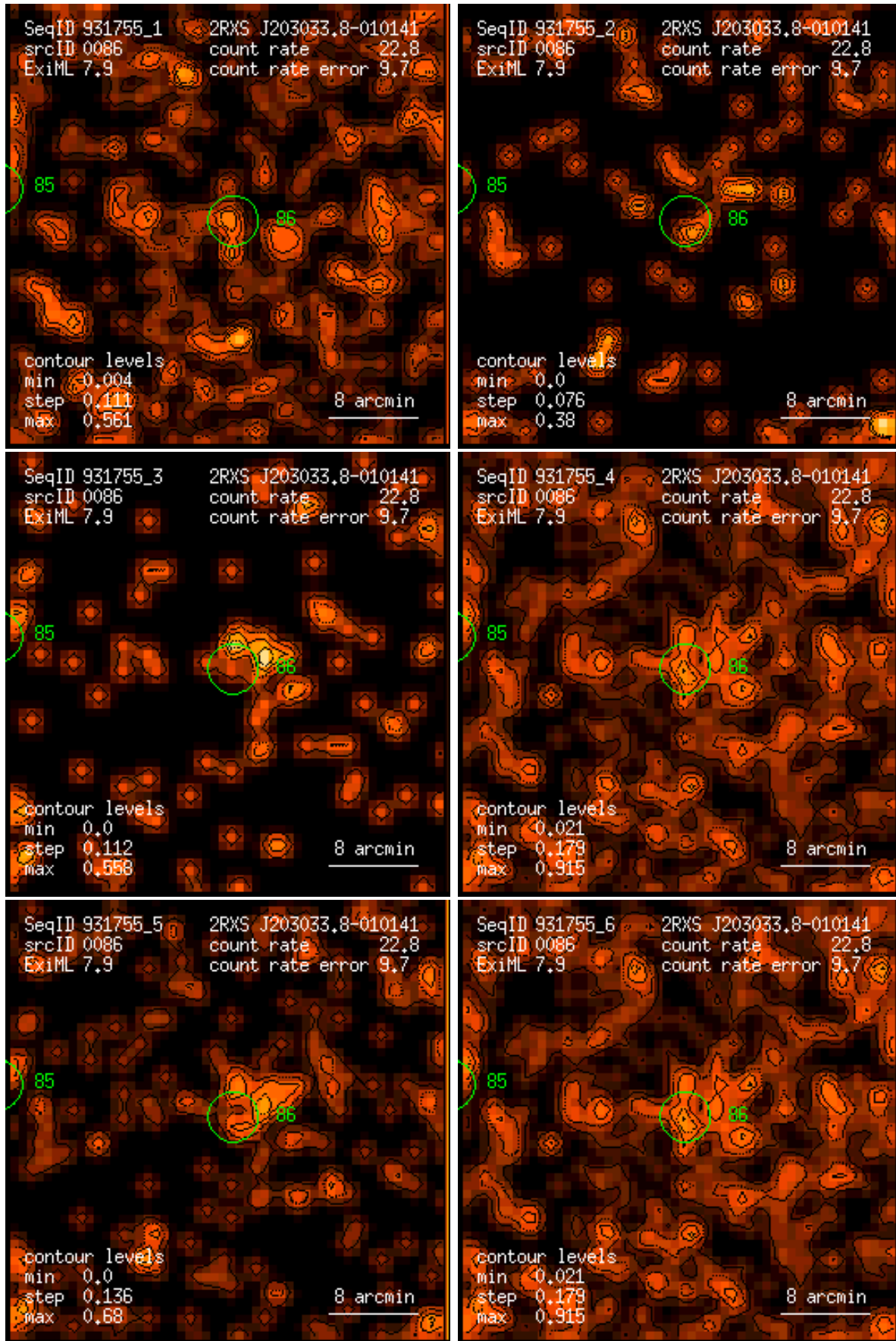
Figure 86: RASS 931755: detection 0086: band rate images, Gaussian filter: (1) PSPC channels 11 – 41, (2) 52 – 90, (3) 91 – 201, (4) 11 – 235, (5) 52 – 201, (6) 11 – 201. Broad band rates in counts/ks. Band rate contour levels in counts/ks/arcmin 2 .
