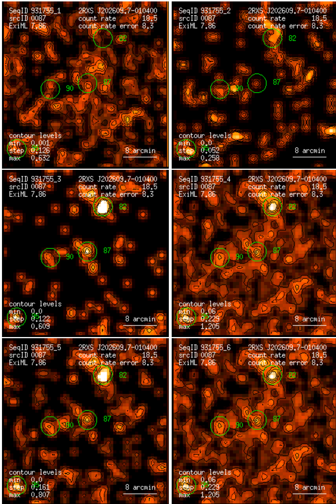
Figure 87: RASS 931755: detection 0087: band rate images, Gaussian filter: (1) PSPC channels 11 – 41, (2) 52 – 90, (3) 91 – 201, (4) 11 – 235, (5) 52 – 201, (6) 11 – 201. Broad band rates in counts/ks. Band rate contour levels in counts/ks/arcmin 2 .
