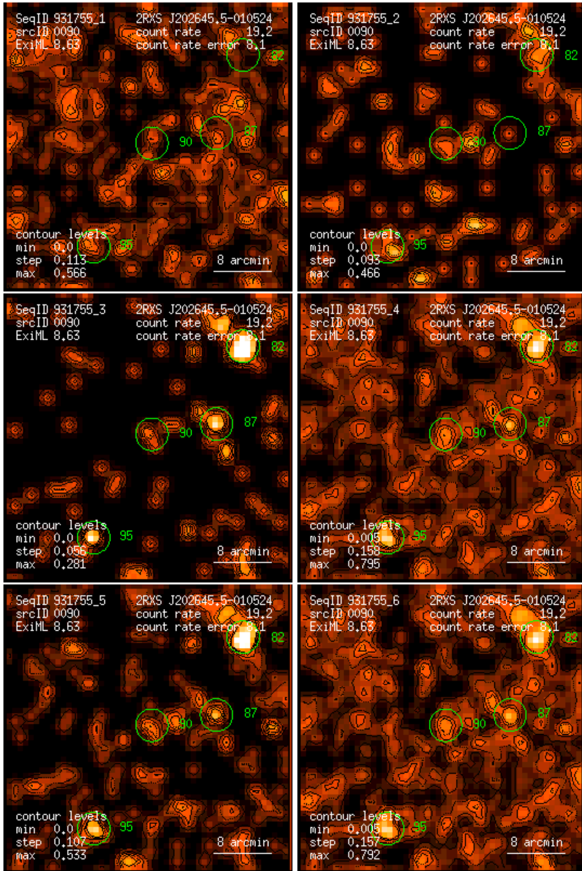
Figure 90: RASS 931755: detection 0090: band rate images, Gaussian filter: (1) PSPC channels 11 – 41, (2) 52 – 90, (3) 91 – 201, (4) 11 – 235, (5) 52 – 201, (6) 11 – 201. Broad band rates in counts/ks. Band rate contour levels in counts/ks/arcmin 2 .
