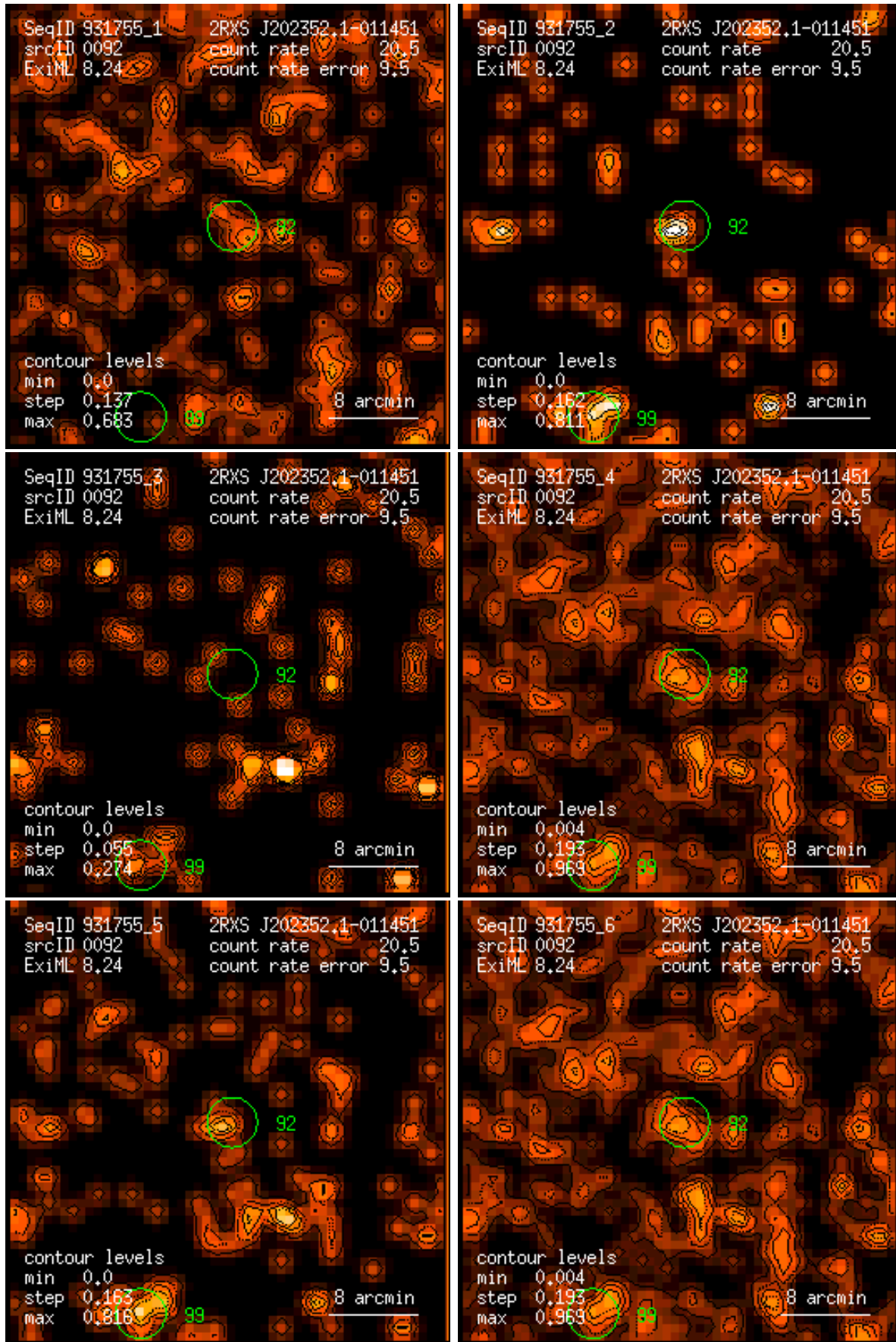
Figure 92: RASS 931755: detection 0092: band rate images, Gaussian filter: (1) PSPC channels 11 – 41, (2) 52 – 90, (3) 91 – 201, (4) 11 – 235, (5) 52 – 201, (6) 11 – 201. Broad band rates in counts/ks. Band rate contour levels in counts/ks/arcmin 2 .
