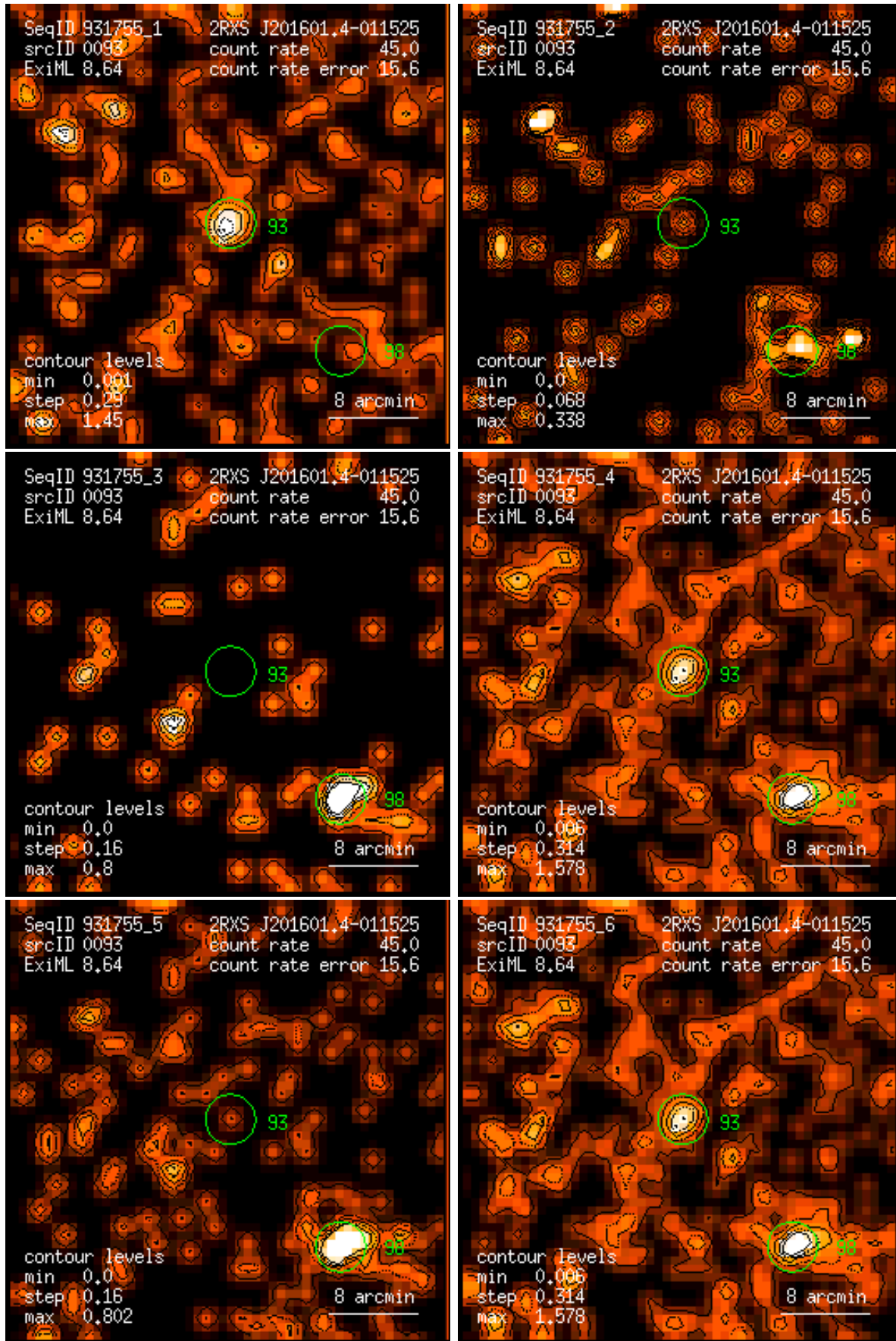
Figure 93: RASS 931755: detection 0093: band rate images, Gaussian filter: (1) PSPC channels 11 – 41, (2) 52 – 90, (3) 91 – 201, (4) 11 – 235, (5) 52 – 201, (6) 11 – 201. Broad band rates in counts/ks. Band rate contour levels in counts/ks/arcmin 2 .
