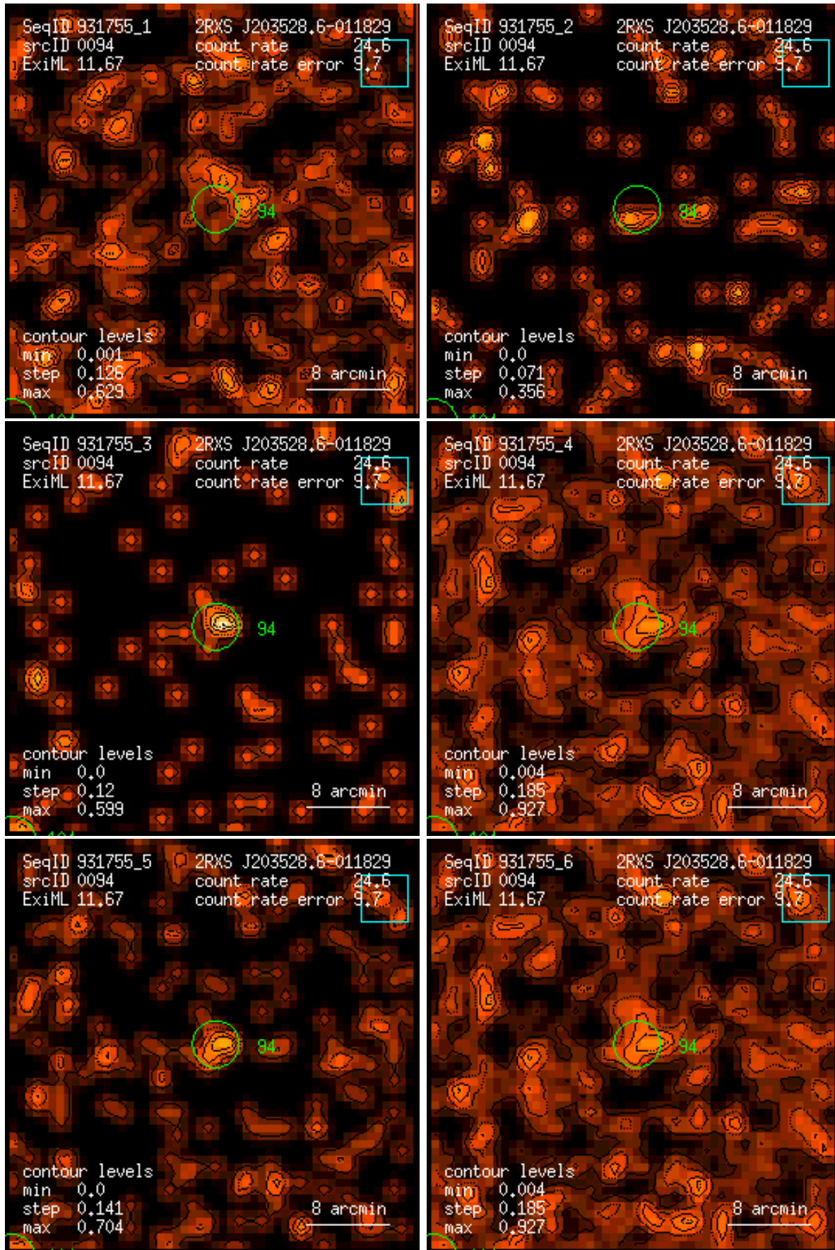
Figure 94: RASS 931755: detection 0094: band rate images, Gaussian filter: (1) PSPC channels 11 – 41, (2) 52 – 90, (3) 91 – 201, (4) 11 – 235, (5) 52 – 201, (6) 11 – 201. Broad band rates in counts/ks. Band rate contour levels in counts/ks/arcmin 2 .
