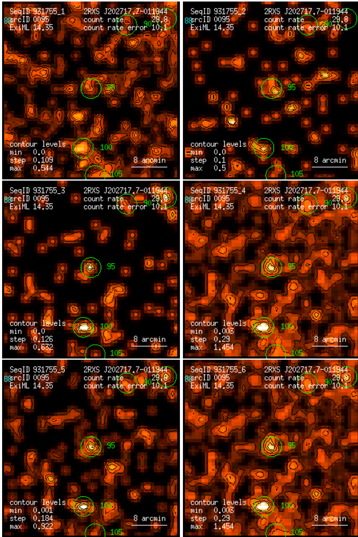
Figure 95: RASS 931755: detection 0095: band rate images, Gaussian filter: (1) PSPC channels 11 – 41, (2) 52 – 90, (3) 91 – 201, (4) 11 – 235, (5) 52 – 201, (6) 11 – 201. Broad band rates in counts/ks. Band rate contour levels in counts/ks/arcmin 2 .
