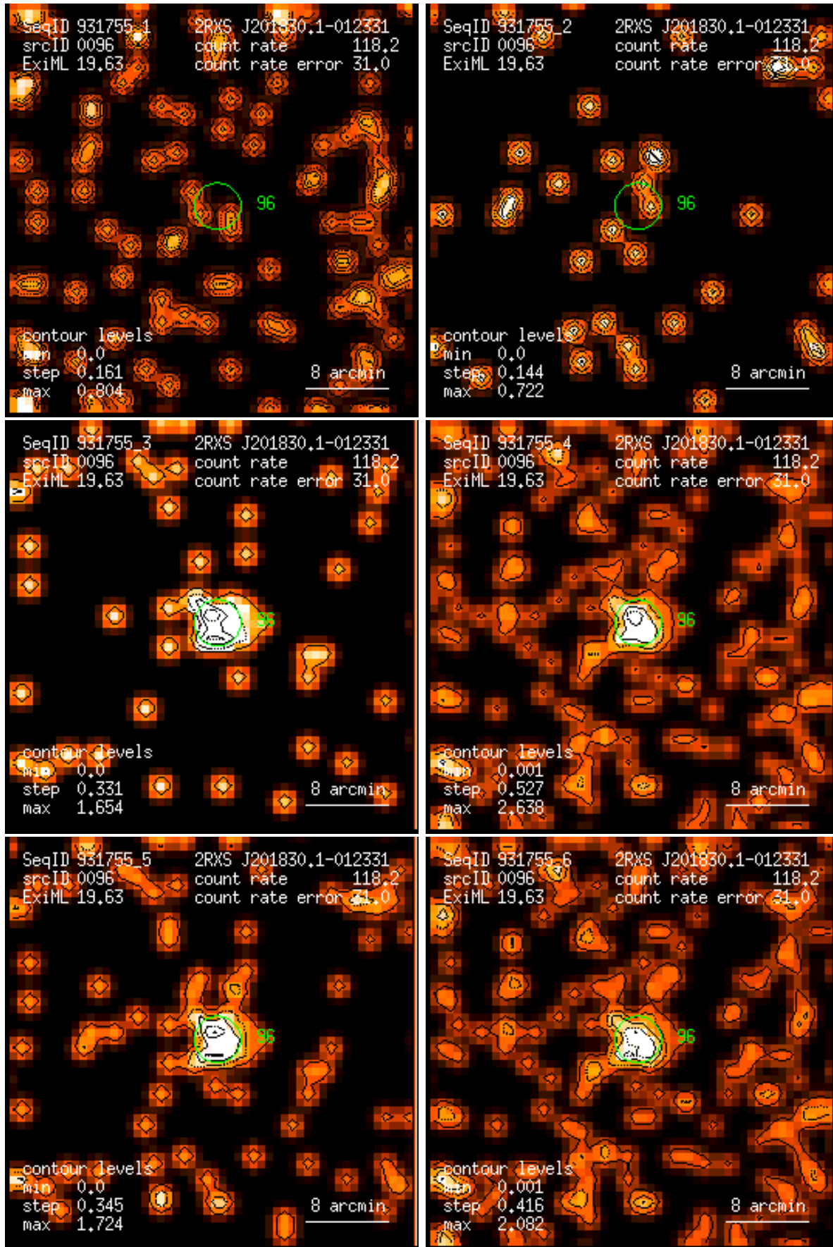
Figure 96: RASS 931755: detection 0096: band rate images, Gaussian filter: (1) PSPC channels 11 – 41, (2) 52 – 90, (3) 91 – 201, (4) 11 – 235, (5) 52 – 201, (6) 11 – 201. Broad band rates in counts/ks. Band rate contour levels in counts/ks/arcmin 2 .
