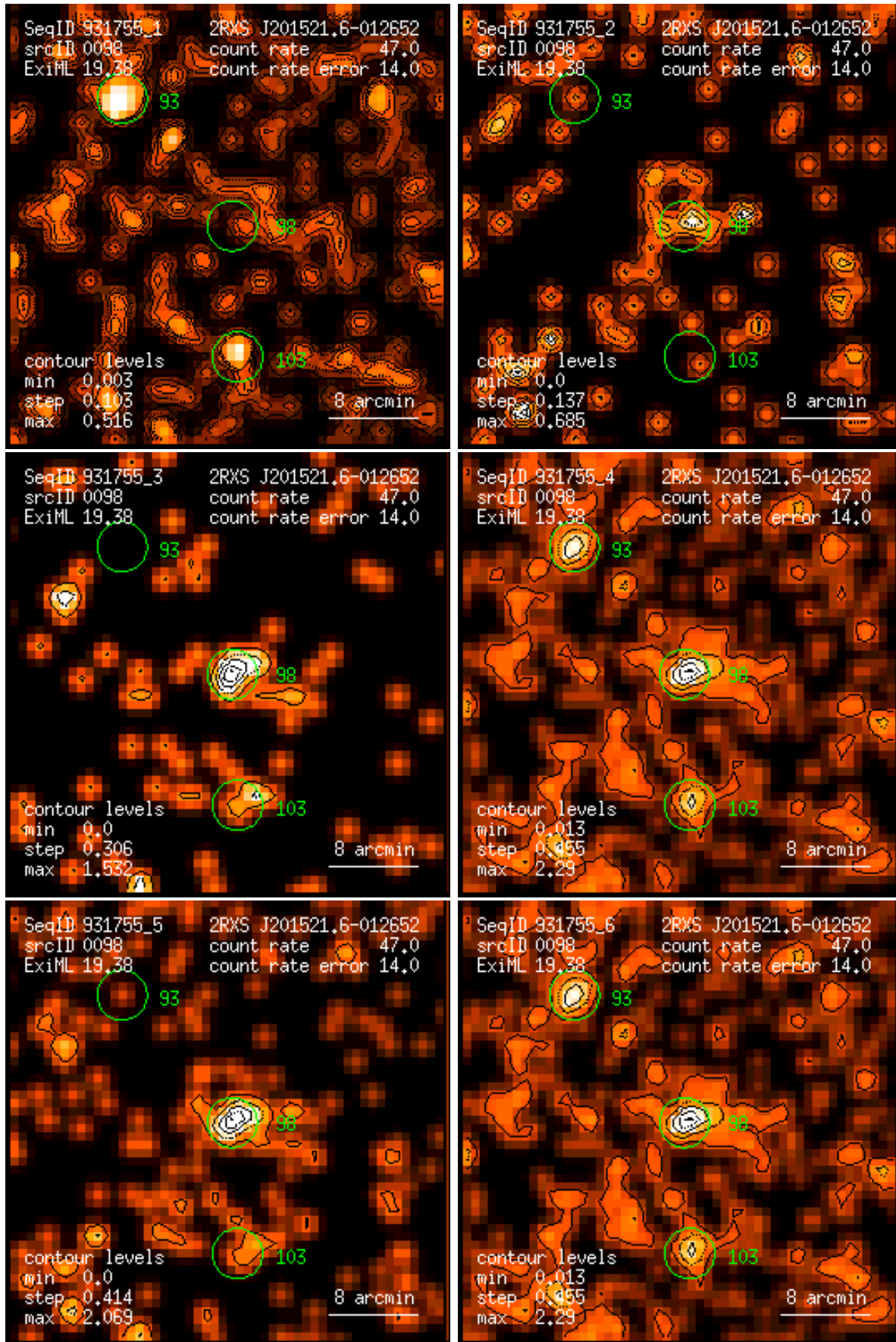
Figure 98: RASS 931755: detection 0098: band rate images, Gaussian filter: (1) PSPC channels 11 – 41, (2) 52 – 90, (3) 91 – 201, (4) 11 – 235, (5) 52 – 201, (6) 11 – 201. Broad band rates in counts/ks. Band rate contour levels in counts/ks/arcmin 2 .
