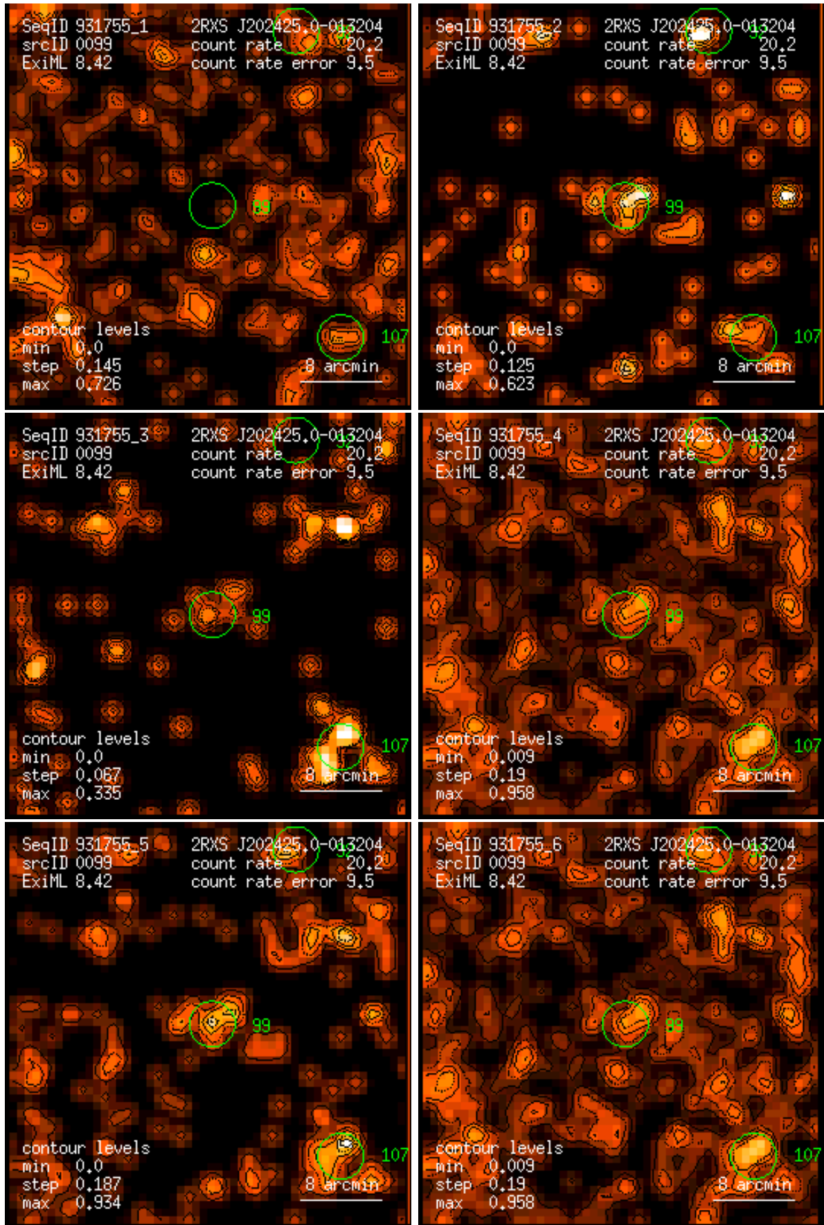
Figure 99: RASS 931755: detection 0099: band rate images, Gaussian filter: (1) PSPC channels 11 – 41, (2) 52 – 90, (3) 91 – 201, (4) 11 – 235, (5) 52 – 201, (6) 11 – 201. Broad band rates in counts/ks. Band rate contour levels in counts/ks/arcmin 2 .
