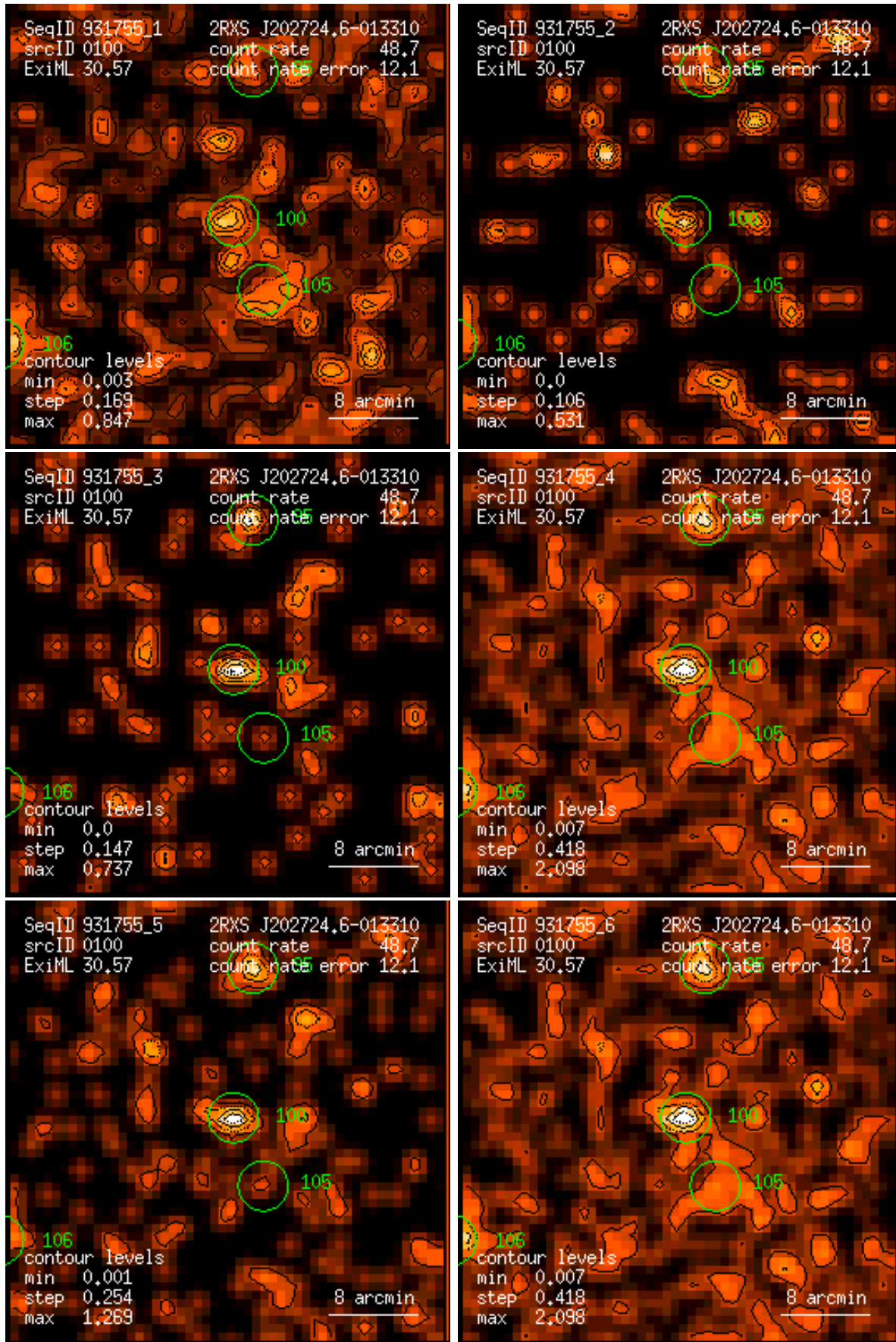
Figure 100: RASS 931755: detection 0100: band rate images, Gaussian filter: (1) PSPC channels 11 – 41, (2) 52 – 90, (3) 91 – 201, (4) 11 – 235, (5) 52 – 201, (6) 11 – 201. Broad band rates in counts/ks. Band rate contour levels in counts/ks/arcmin 2 .
