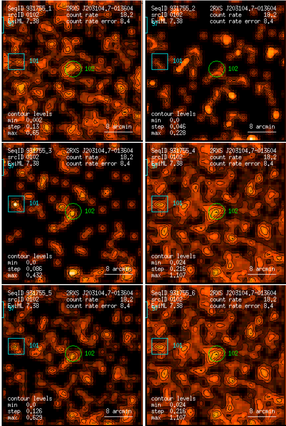
Figure 102: RASS 931755: detection 0102: band rate images, Gaussian filter: (1) PSPC channels 11 – 41, (2) 52 – 90, (3) 91 – 201, (4) 11 – 235, (5) 52 – 201, (6) 11 – 201. Broad band rates in counts/ks. Band rate contour levels in counts/ks/arcmin 2 .
