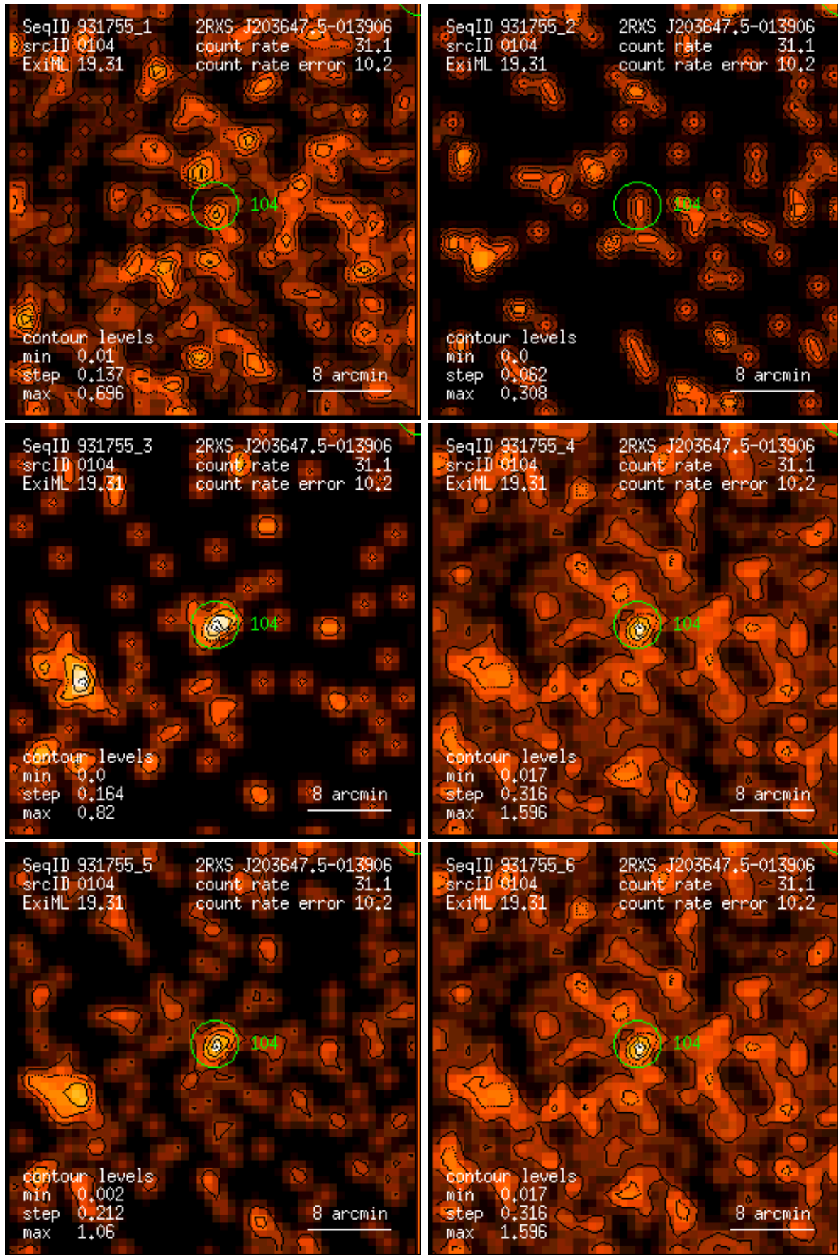
Figure 104: RASS 931755: detection 0104: band rate images, Gaussian filter: (1) PSPC channels 11 – 41, (2) 52 – 90, (3) 91 – 201, (4) 11 – 235, (5) 52 – 201, (6) 11 – 201. Broad band rates in counts/ks. Band rate contour levels in counts/ks/arcmin 2 .
