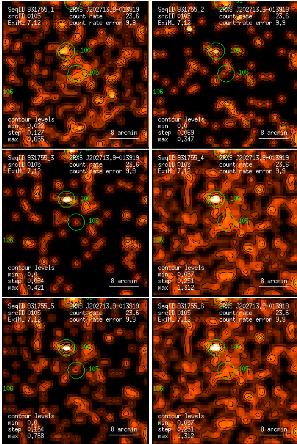
Figure 105: RASS 931755: detection 0105: band rate images, Gaussian filter: (1) PSPC channels 11 – 41, (2) 52 – 90, (3) 91 – 201, (4) 11 – 235, (5) 52 – 201, (6) 11 – 201. Broad band rates in counts/ks. Band rate contour levels in counts/ks/arcmin 2 .
