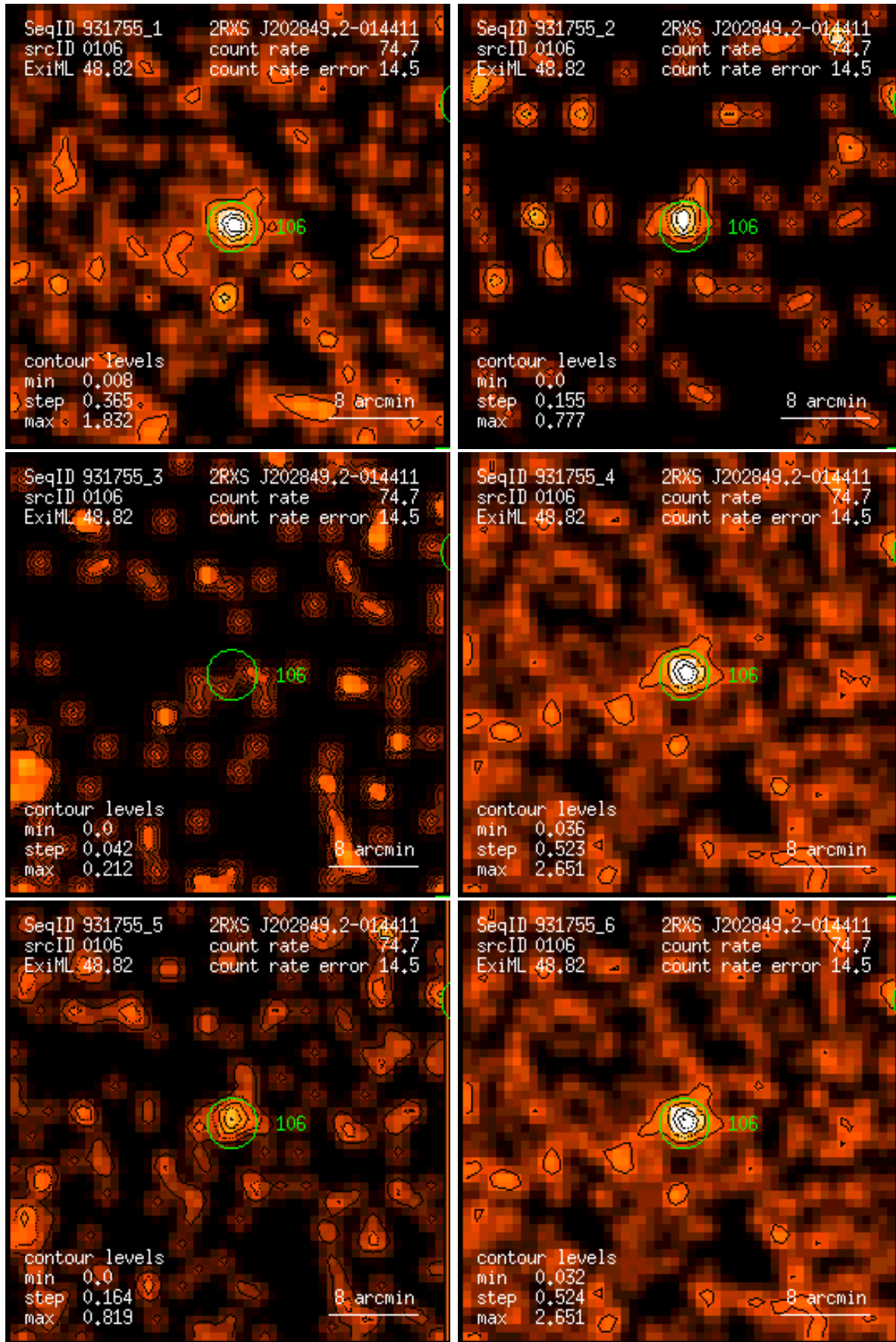
Figure 106: RASS 931755: detection 0106: band rate images, Gaussian filter: (1) PSPC channels 11 – 41, (2) 52 – 90, (3) 91 – 201, (4) 11 – 235, (5) 52 – 201, (6) 11 – 201. Broad band rates in counts/ks. Band rate contour levels in counts/ks/arcmin 2 .
