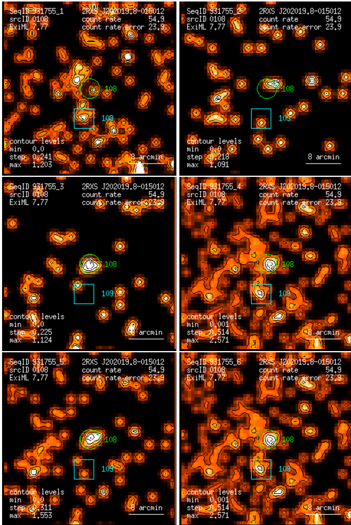
Figure 108: RASS 931755: detection 0108: band rate images, Gaussian filter: (1) PSPC channels 11 – 41, (2) 52 – 90, (3) 91 – 201, (4) 11 – 235, (5) 52 – 201, (6) 11 – 201. Broad band rates in counts/ks. Band rate contour levels in counts/ks/arcmin 2 .
