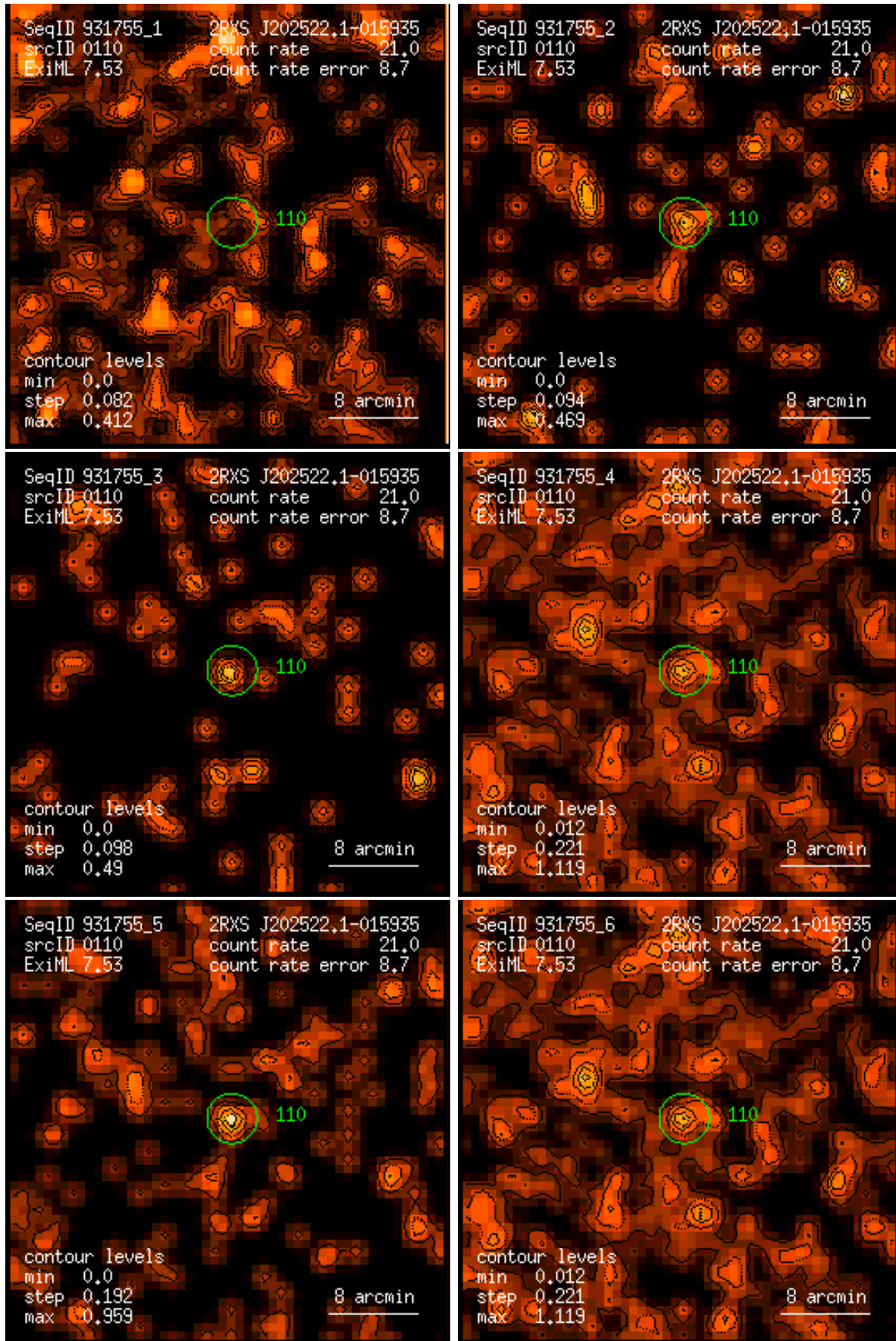
Figure 110: RASS 931755: detection 0110: band rate images, Gaussian filter: (1) PSPC channels 11 – 41, (2) 52 – 90, (3) 91 – 201, (4) 11 – 235, (5) 52 – 201, (6) 11 – 201. Broad band rates in counts/ks. Band rate contour levels in counts/ks/arcmin 2 .
