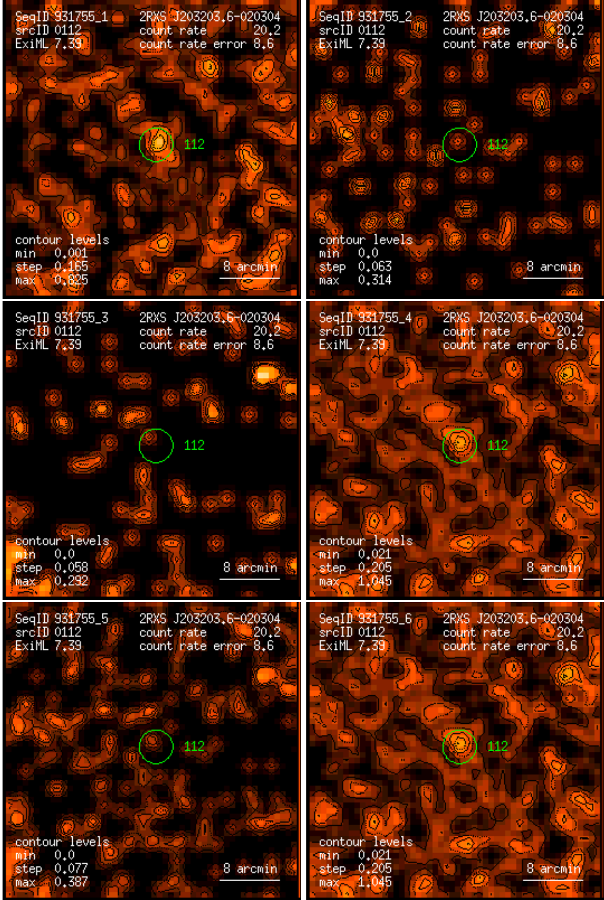
Figure 112: RASS 931755: detection 0112: band rate images, Gaussian filter: (1) PSPC channels 11 – 41, (2) 52 – 90, (3) 91 – 201, (4) 11 – 235, (5) 52 – 201, (6) 11 – 201. Broad band rates in counts/ks. Band rate contour levels in counts/ks/arcmin 2 .
