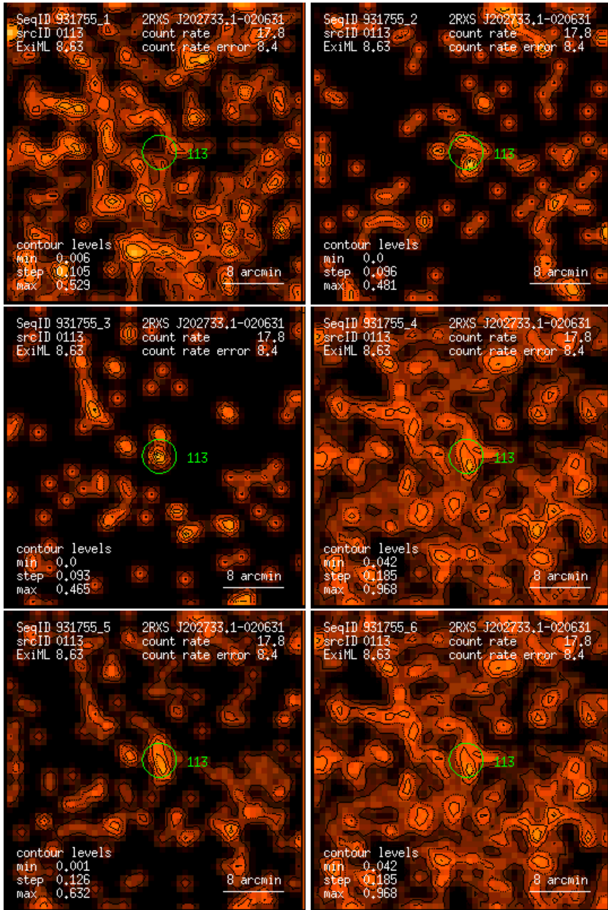
Figure 113: RASS 931755: detection 0113: band rate images, Gaussian filter: (1) PSPC channels 11 – 41, (2) 52 – 90, (3) 91 – 201, (4) 11 – 235, (5) 52 – 201, (6) 11 – 201. Broad band rates in counts/ks. Band rate contour levels in counts/ks/arcmin 2 .
