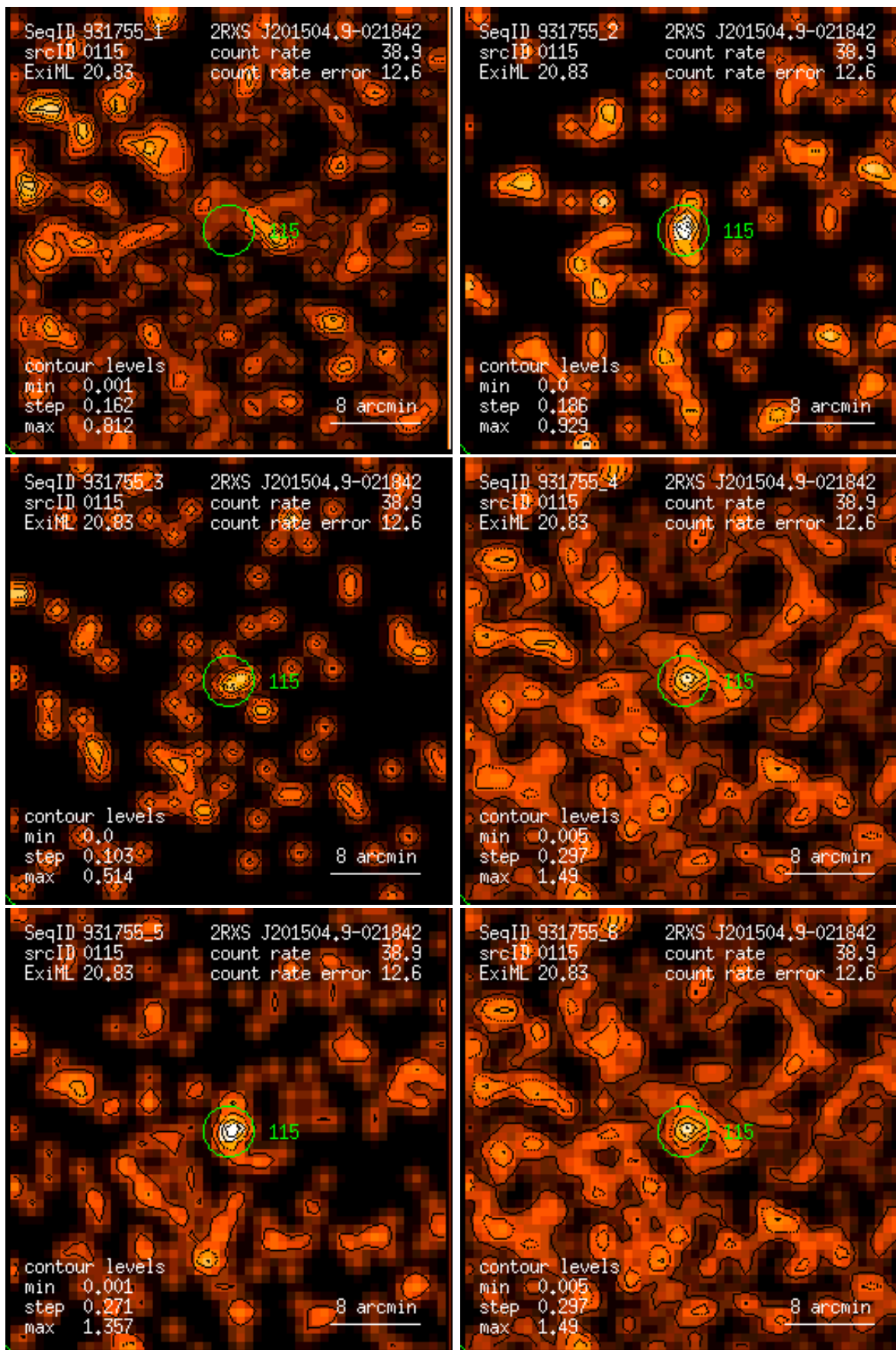
Figure 115: RASS 931755: detection 0115: band rate images, Gaussian filter: (1) PSPC channels 11 – 41, (2) 52 – 90, (3) 91 – 201, (4) 11 – 235, (5) 52 – 201, (6) 11 – 201. Broad band rates in counts/ks. Band rate contour levels in counts/ks/arcmin 2 .
