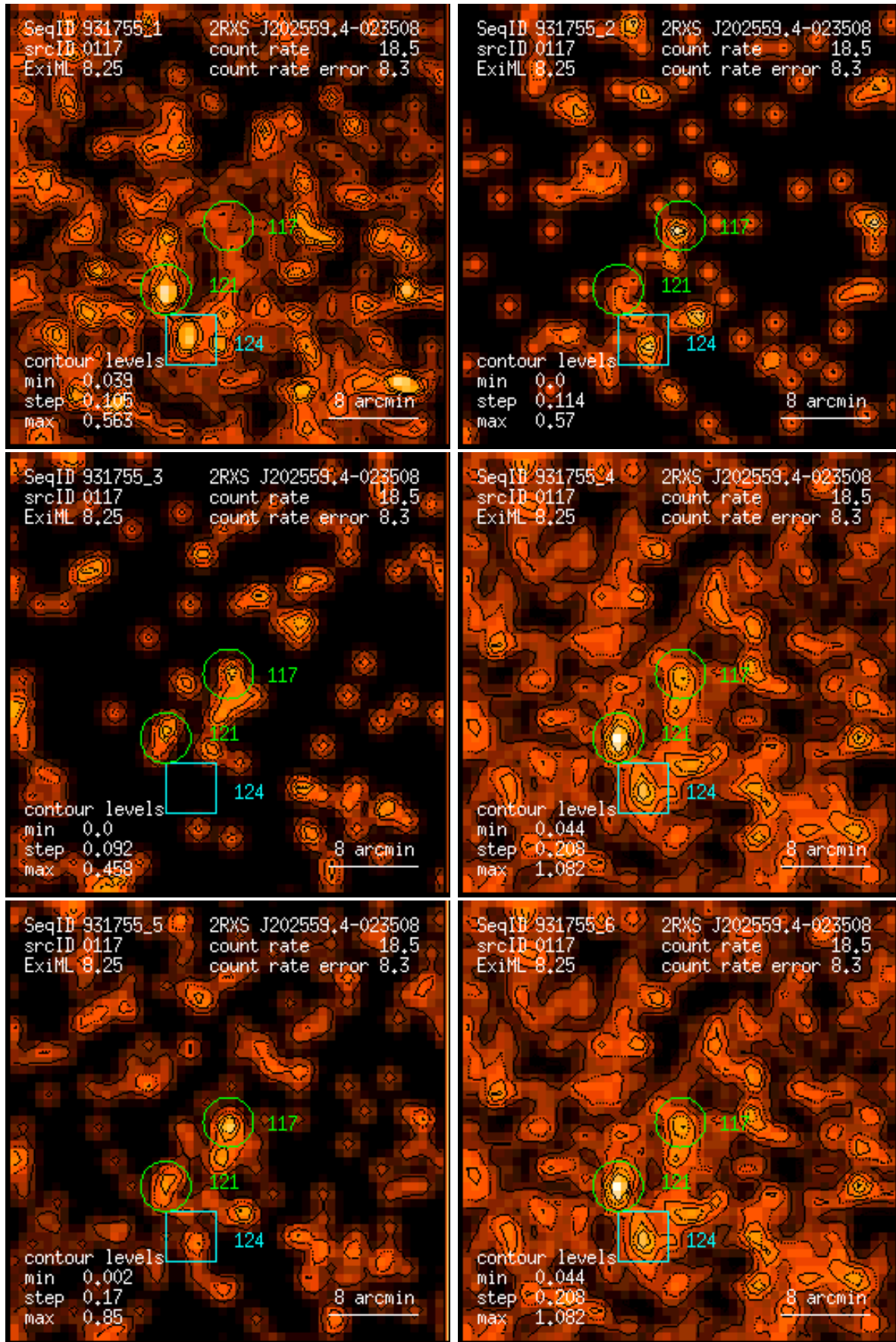
Figure 117: RASS 931755: detection 0117: band rate images, Gaussian filter: (1) PSPC channels 11 – 41, (2) 52 – 90, (3) 91 – 201, (4) 11 – 235, (5) 52 – 201, (6) 11 – 201. Broad band rates in counts/ks. Band rate contour levels in counts/ks/arcmin 2 .
