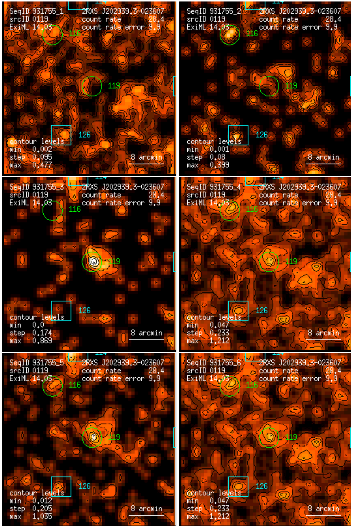
Figure 119: RASS 931755: detection 0119: band rate images, Gaussian filter: (1) PSPC channels 11 – 41, (2) 52 – 90, (3) 91 – 201, (4) 11 – 235, (5) 52 – 201, (6) 11 – 201. Broad band rates in counts/ks. Band rate contour levels in counts/ks/arcmin 2 .
